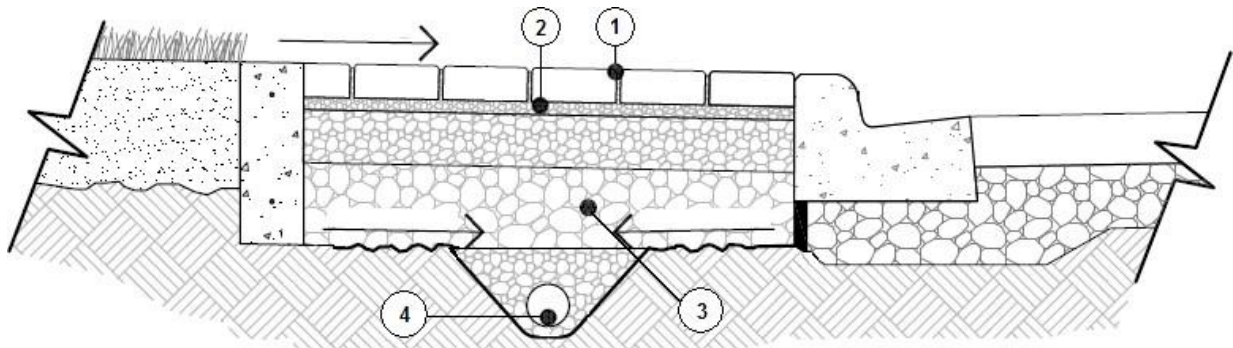
Figure 4.7: Components of permeable pavement facilities
