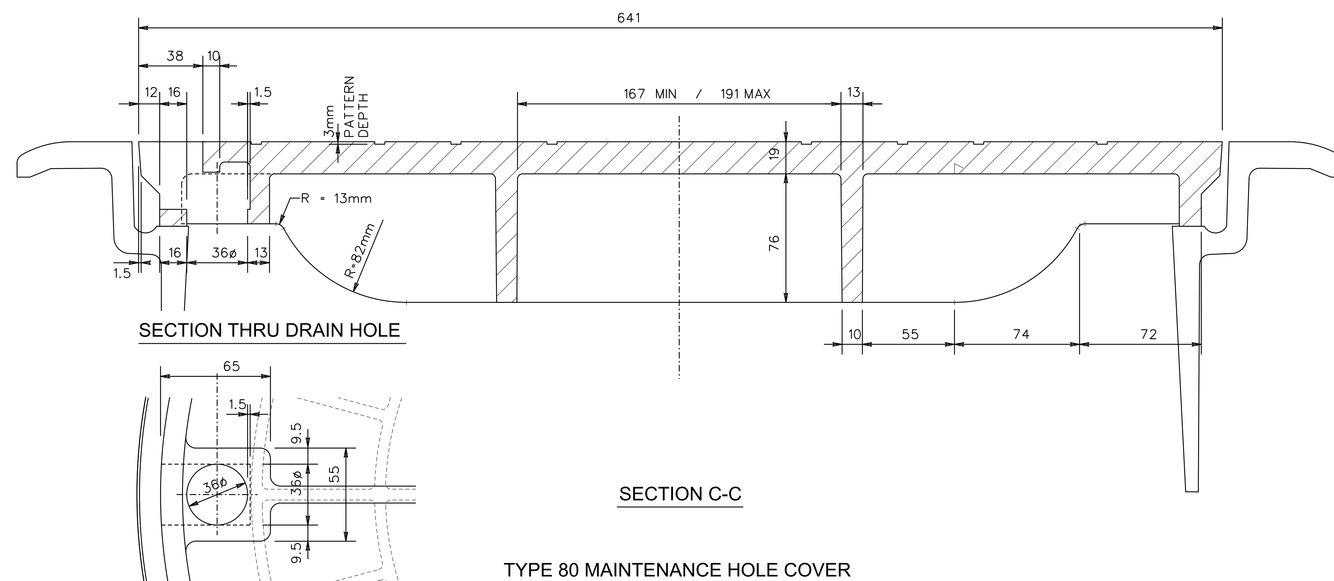
DRAIN HOLE DETAIL BOTTOM VIEW
