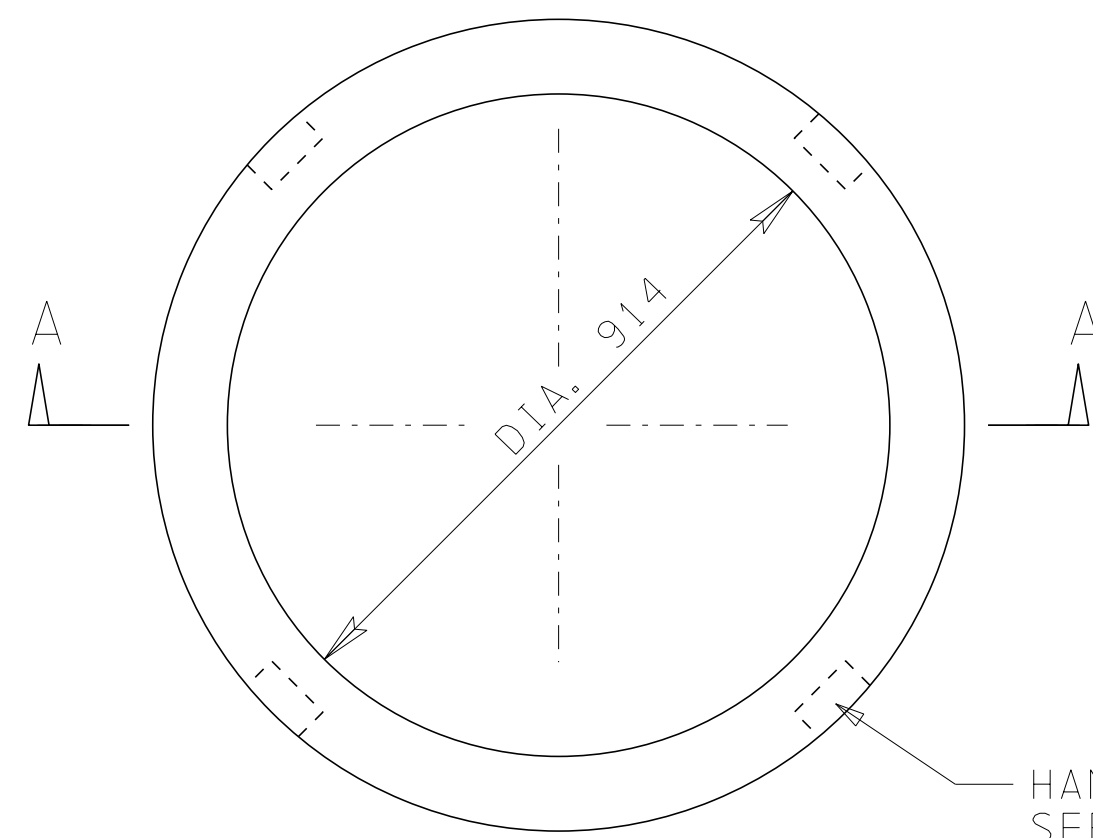
PLAN VIEW
