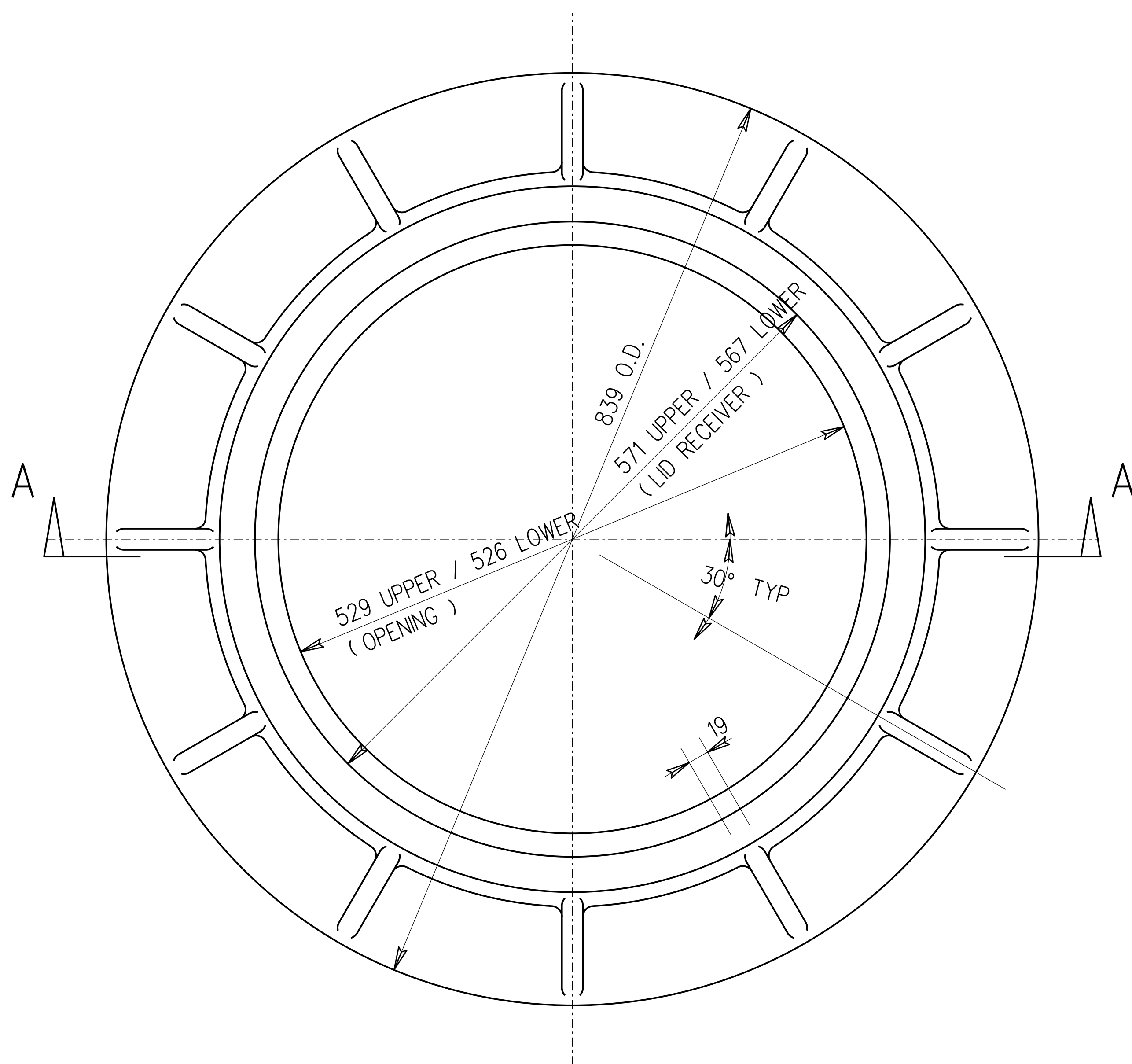
TOP VIEW
