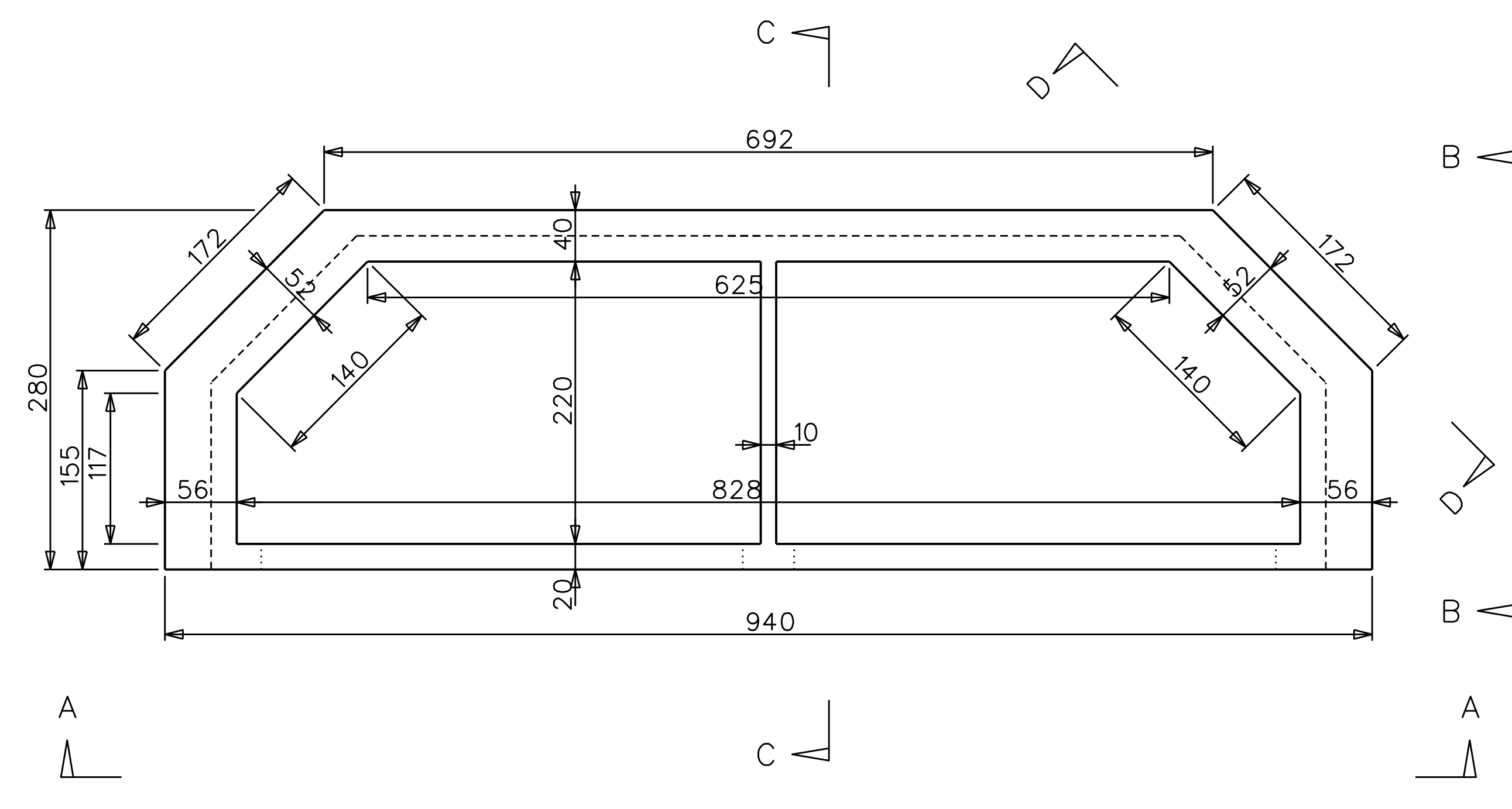
PLAN VIEW - BOTTOM
