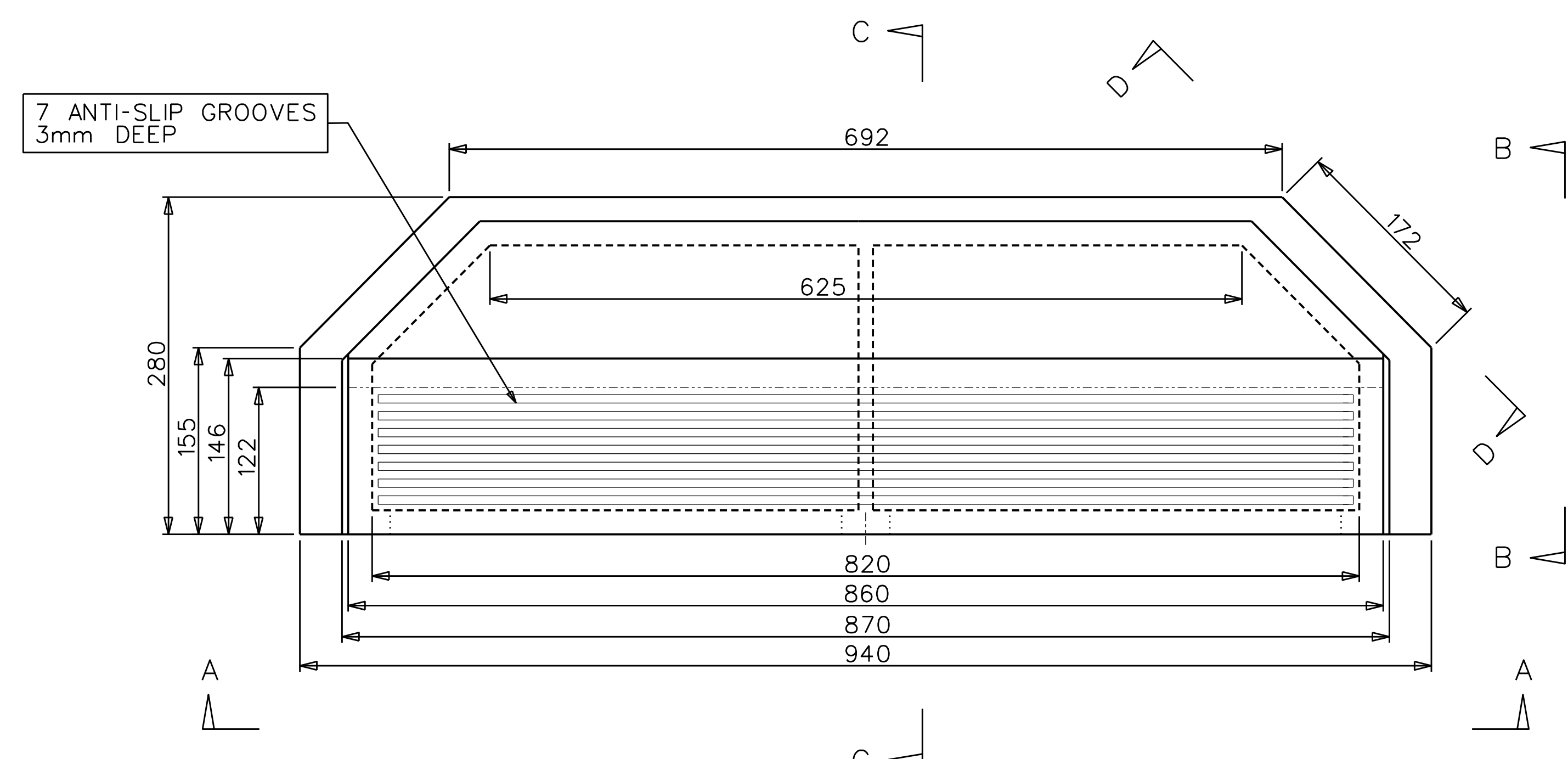
SIDE INLET
