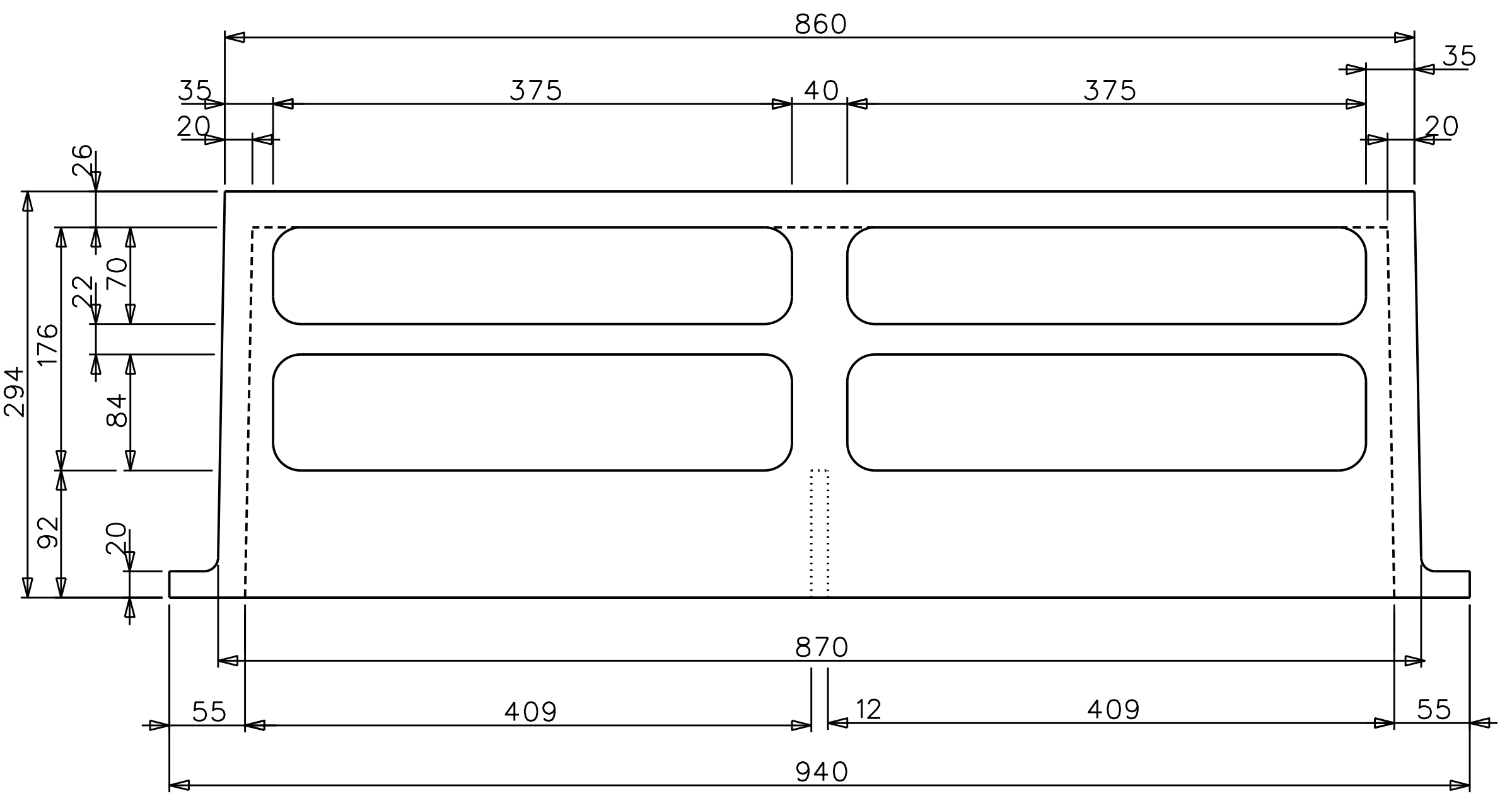
FRONT VIEW A - A
