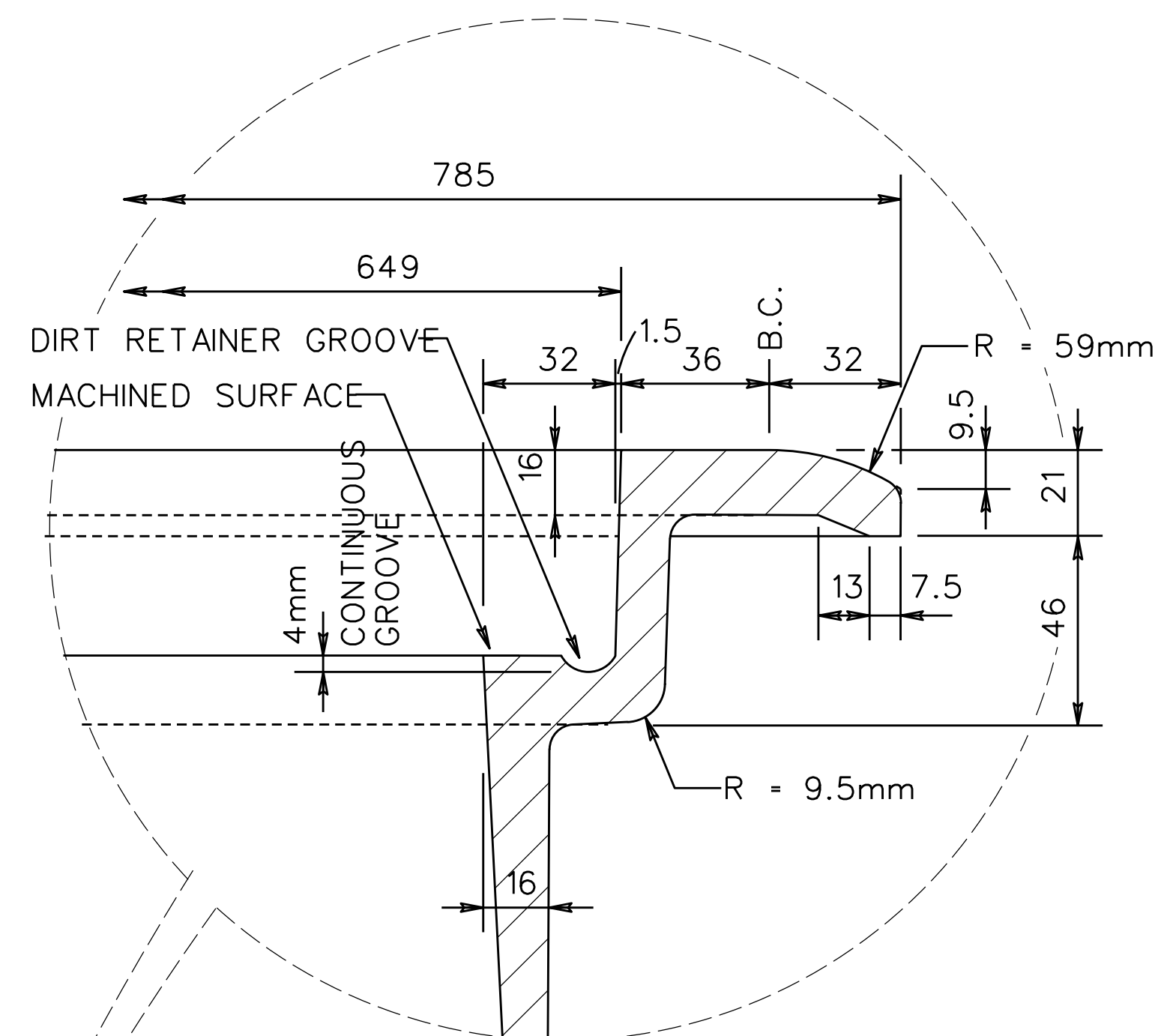
DETAIL SCALE 1:2
