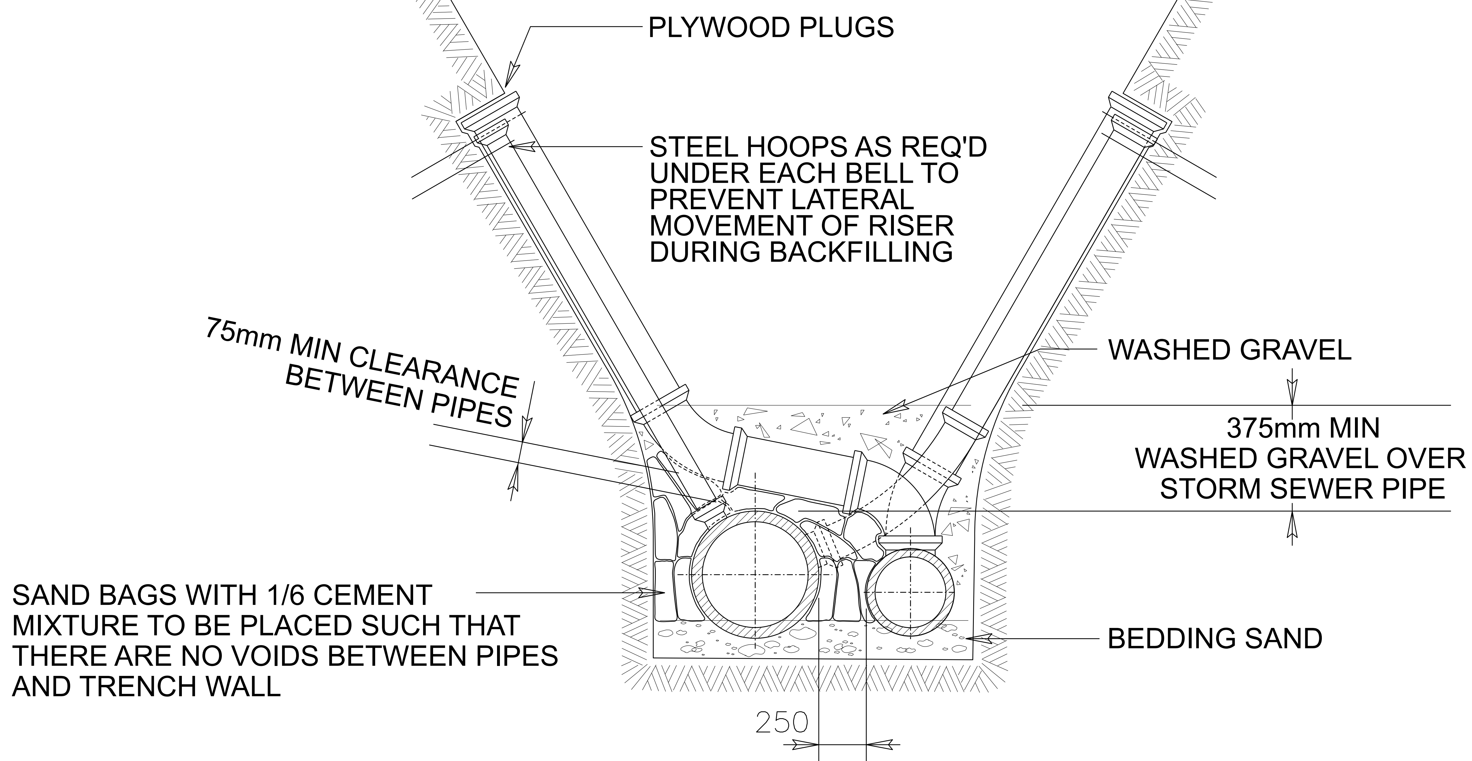
SECTION A - A
