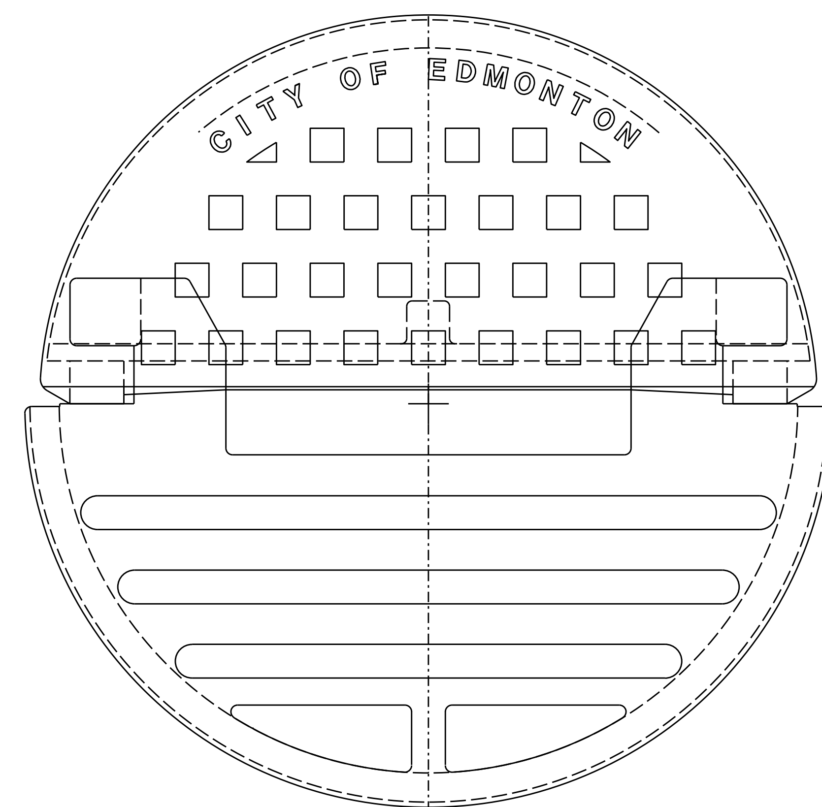
PLAN VIEW COVER COMPONENTS ASSEMBLED
