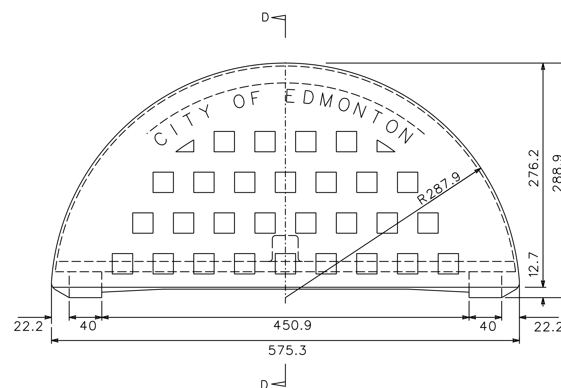
TOP VIEW - COVER (Part B)
