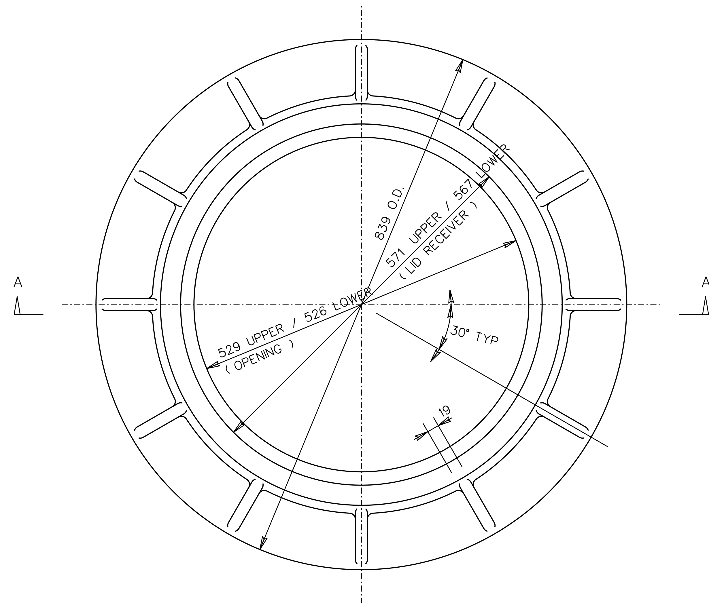
TOP VIEW
