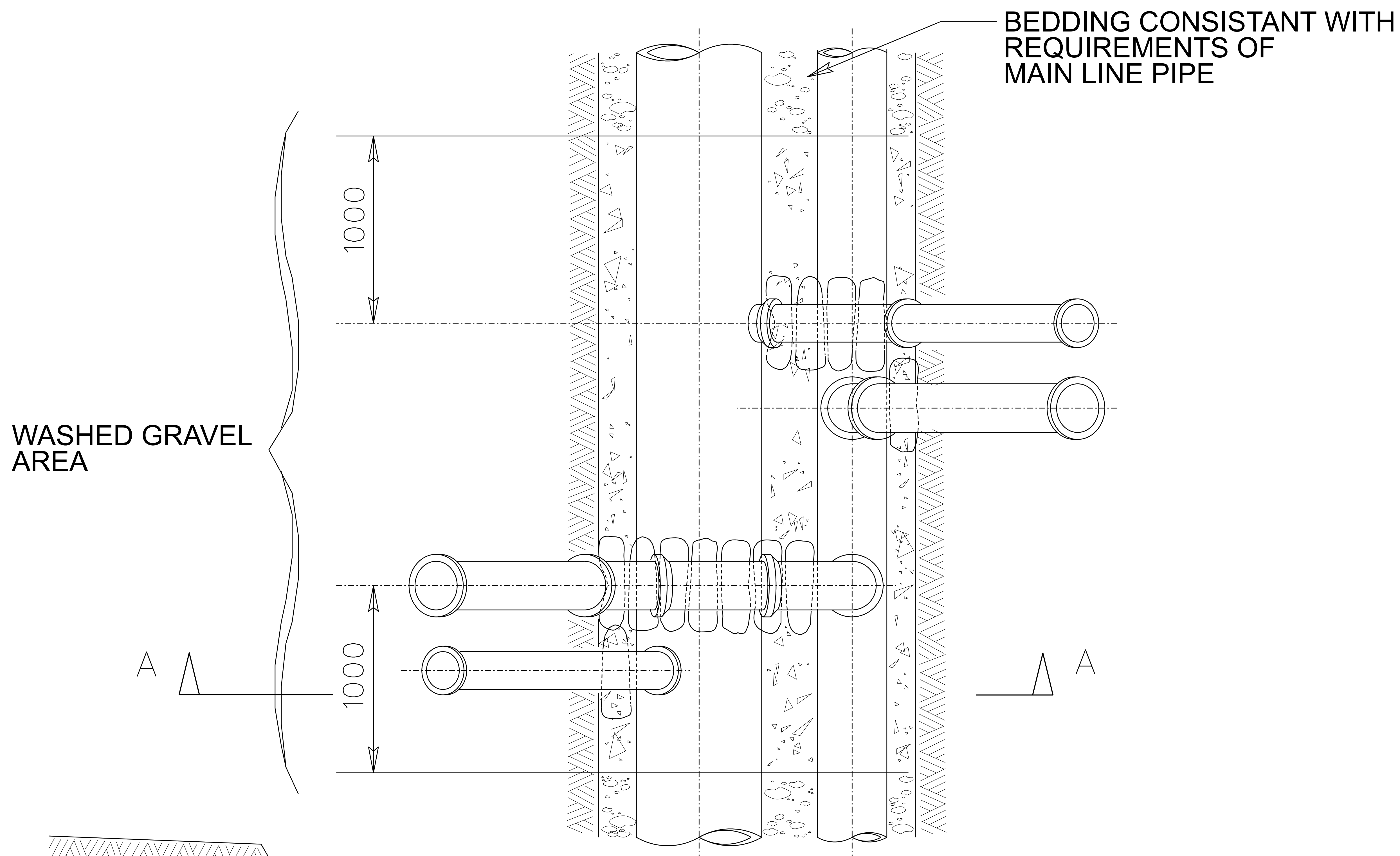
PLAN
