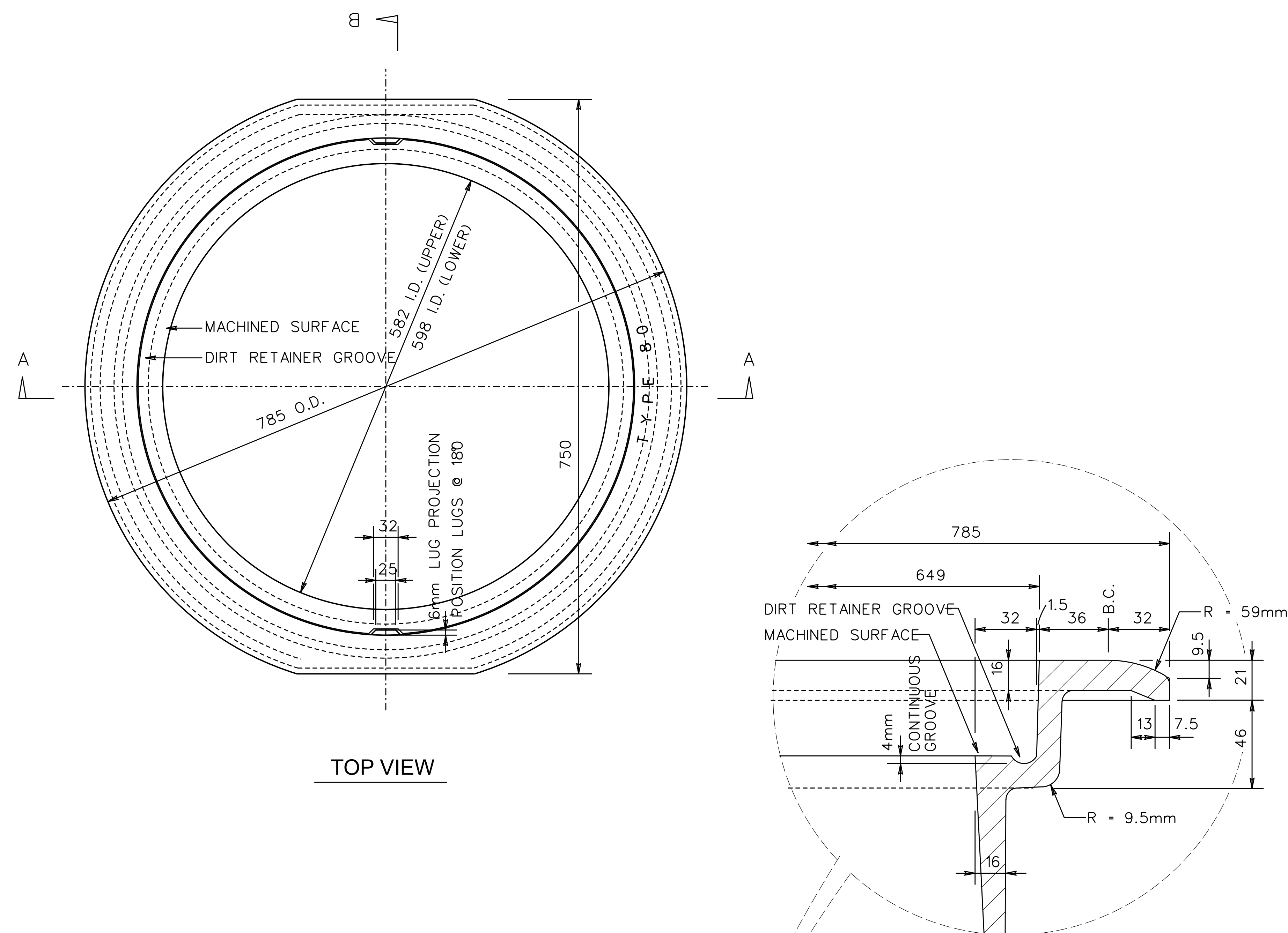
DETAIL SCALE 1:2
