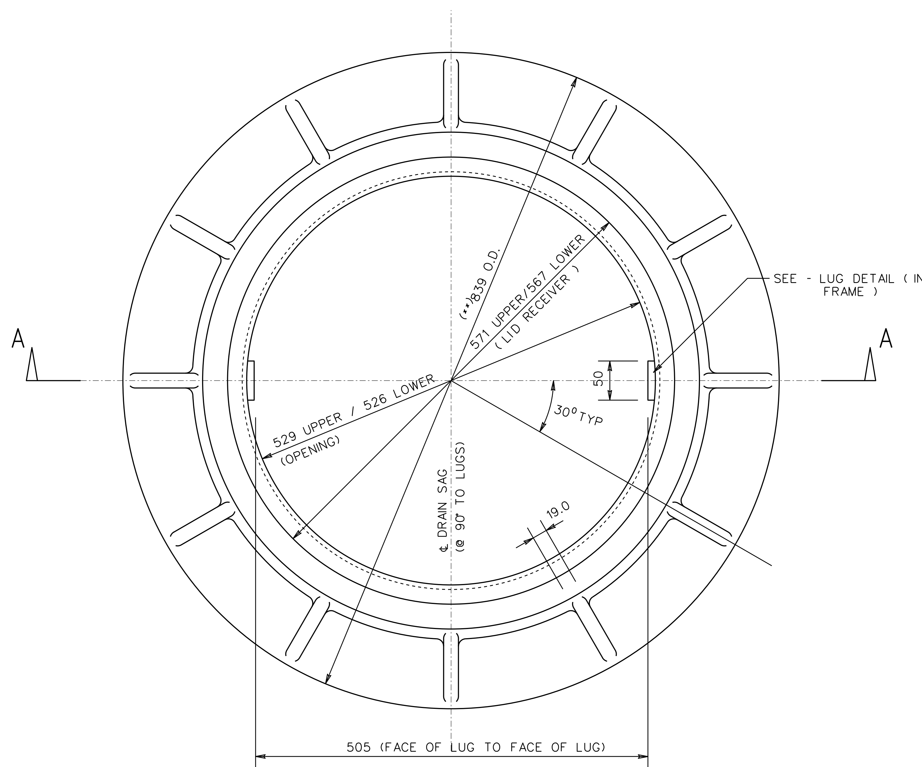
TOP VIEW
