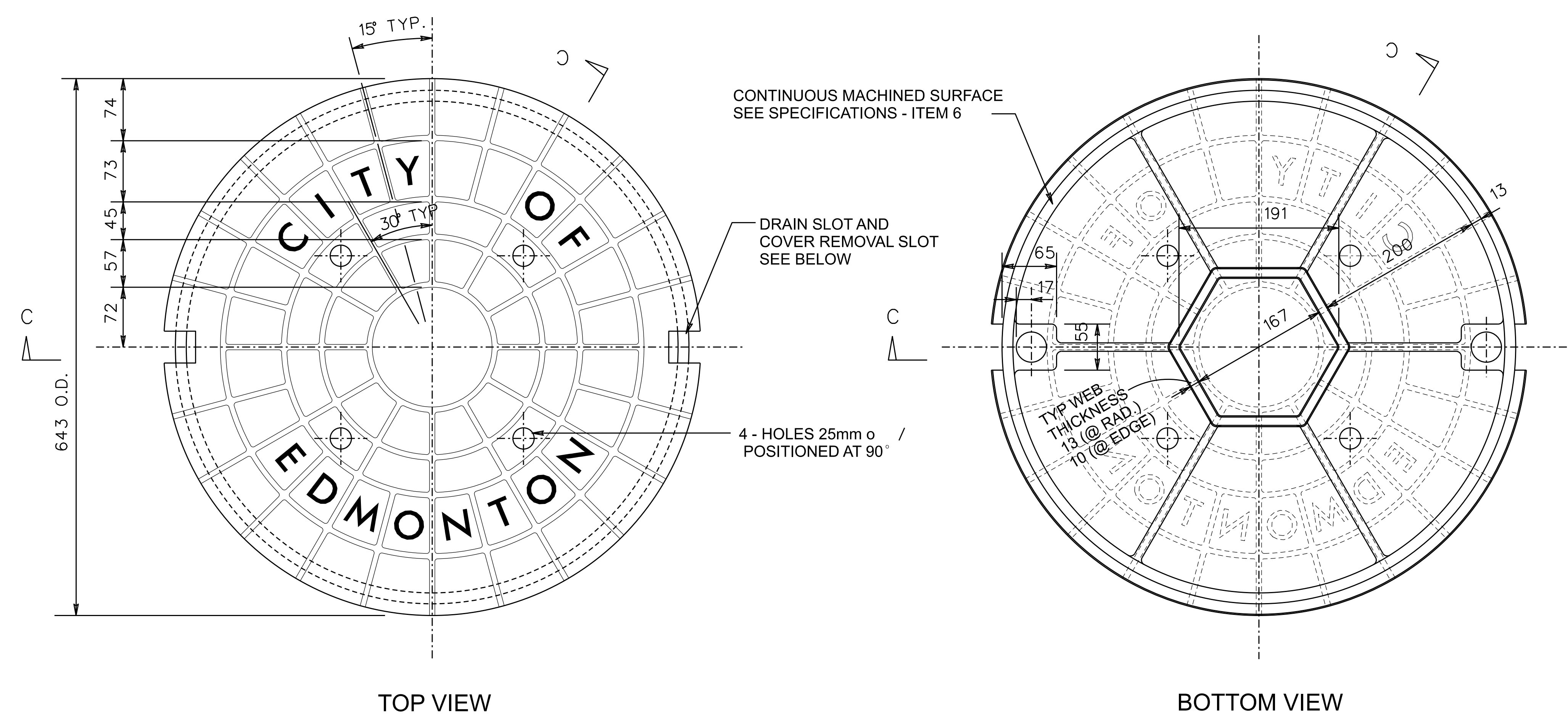
TOP VIEW
