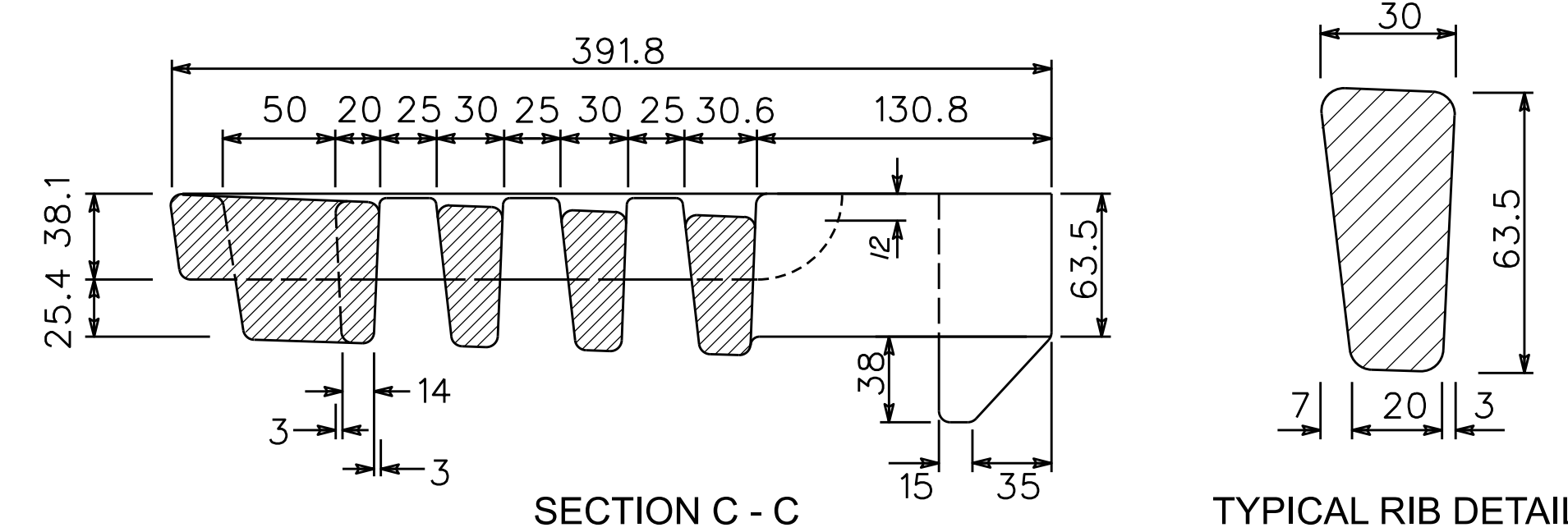
TYPICAL RIB DETAIL
