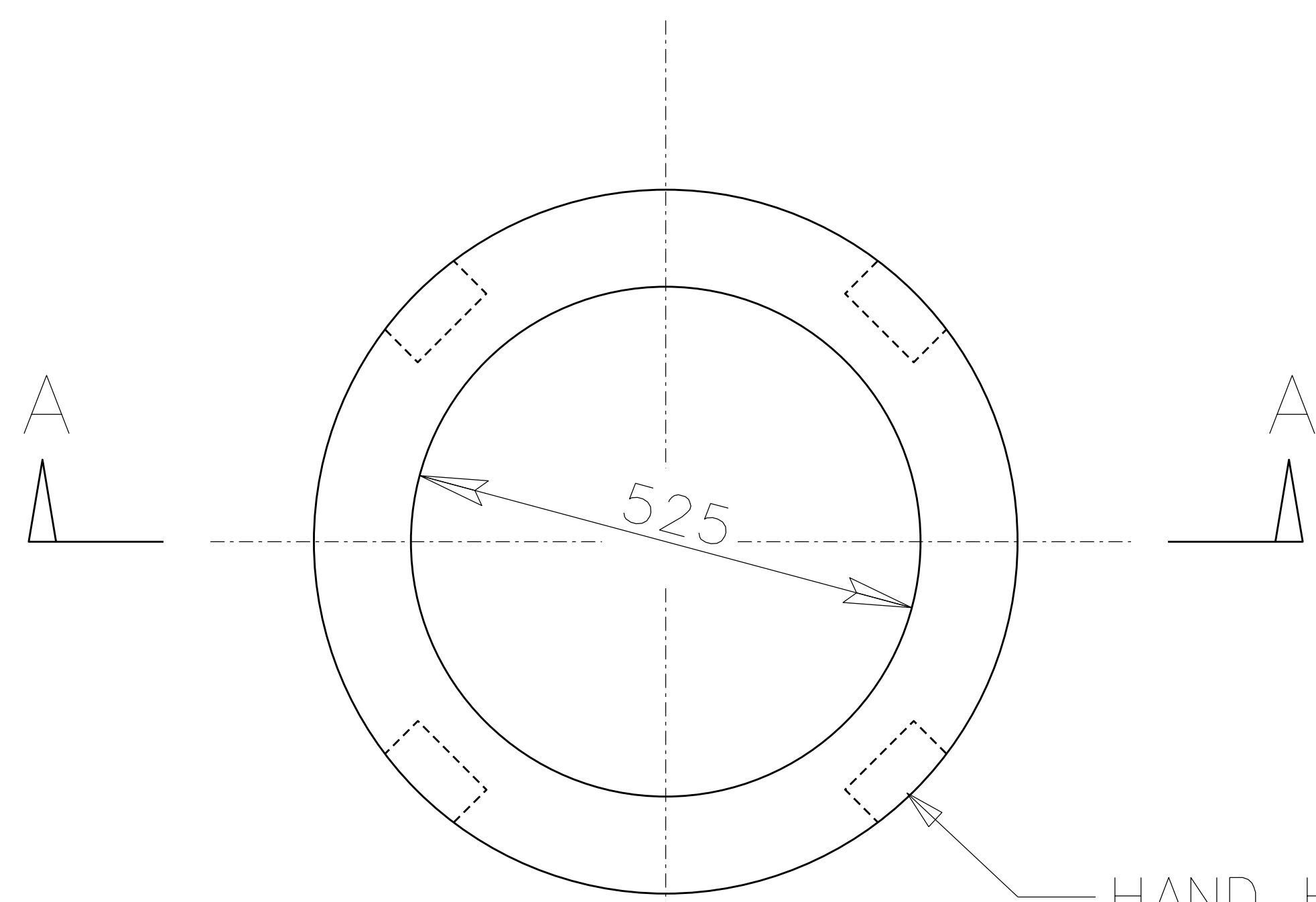
PLAN VIEW
