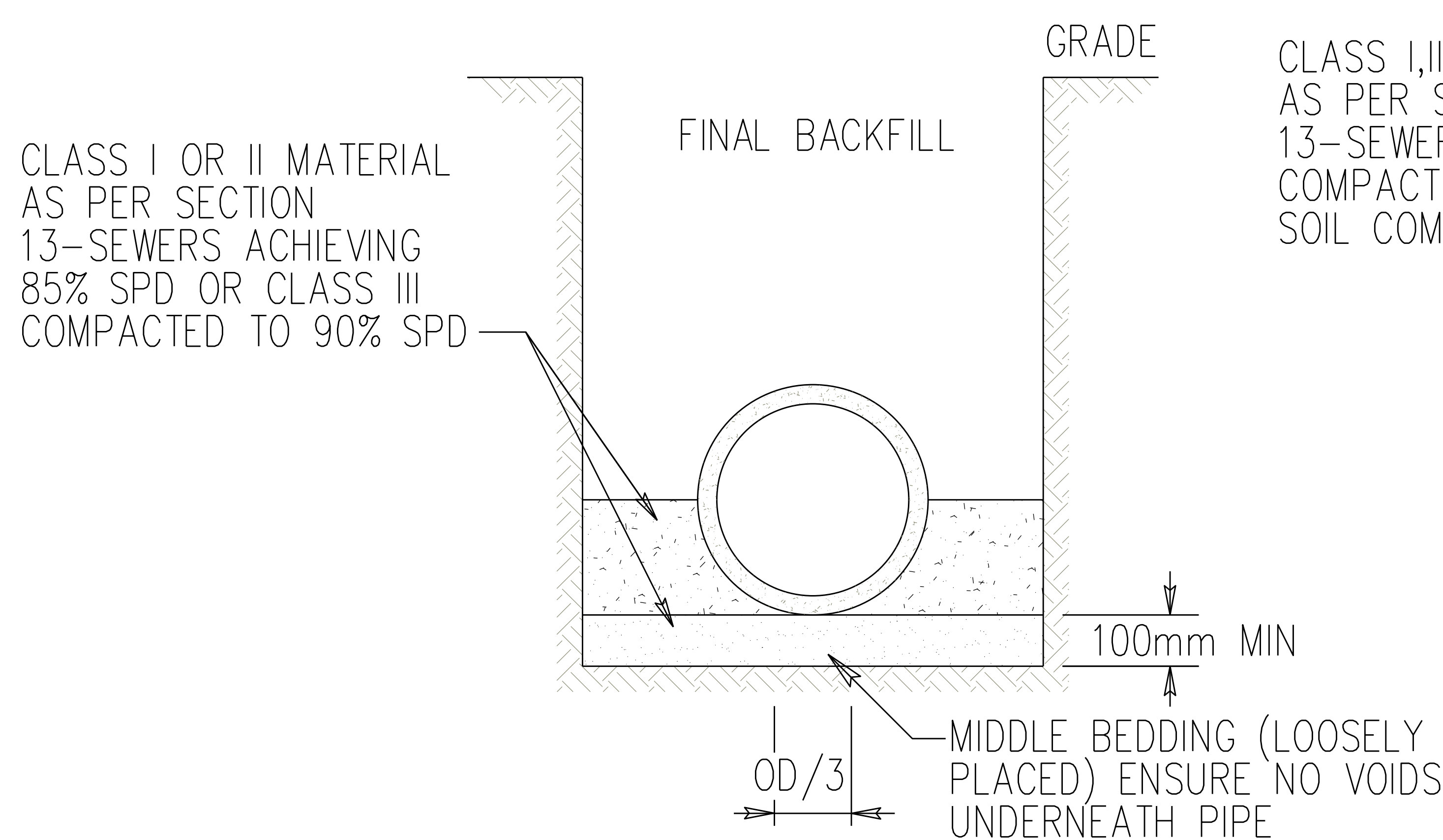
TYPE 3 INSTALLATION
