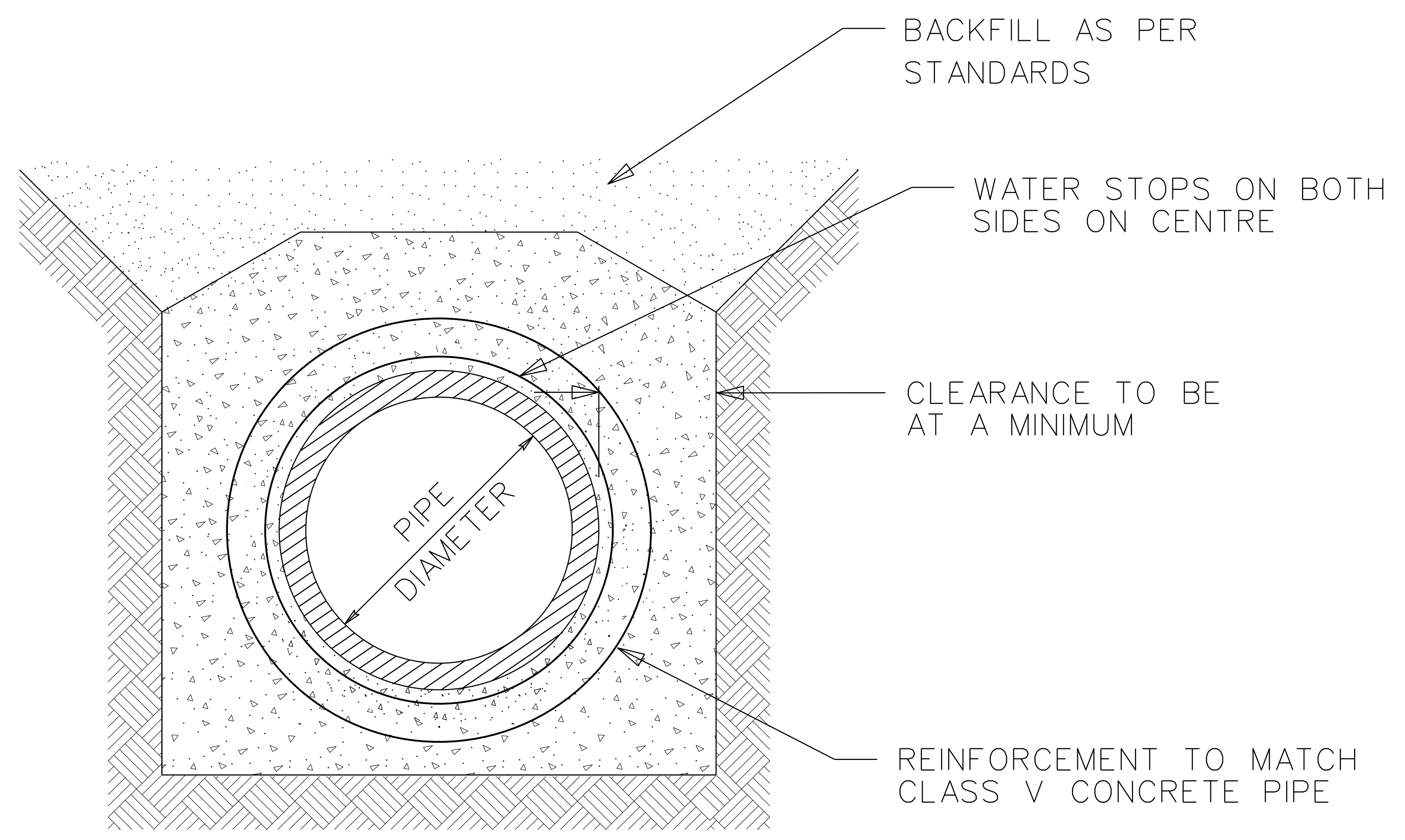
END VIEW
