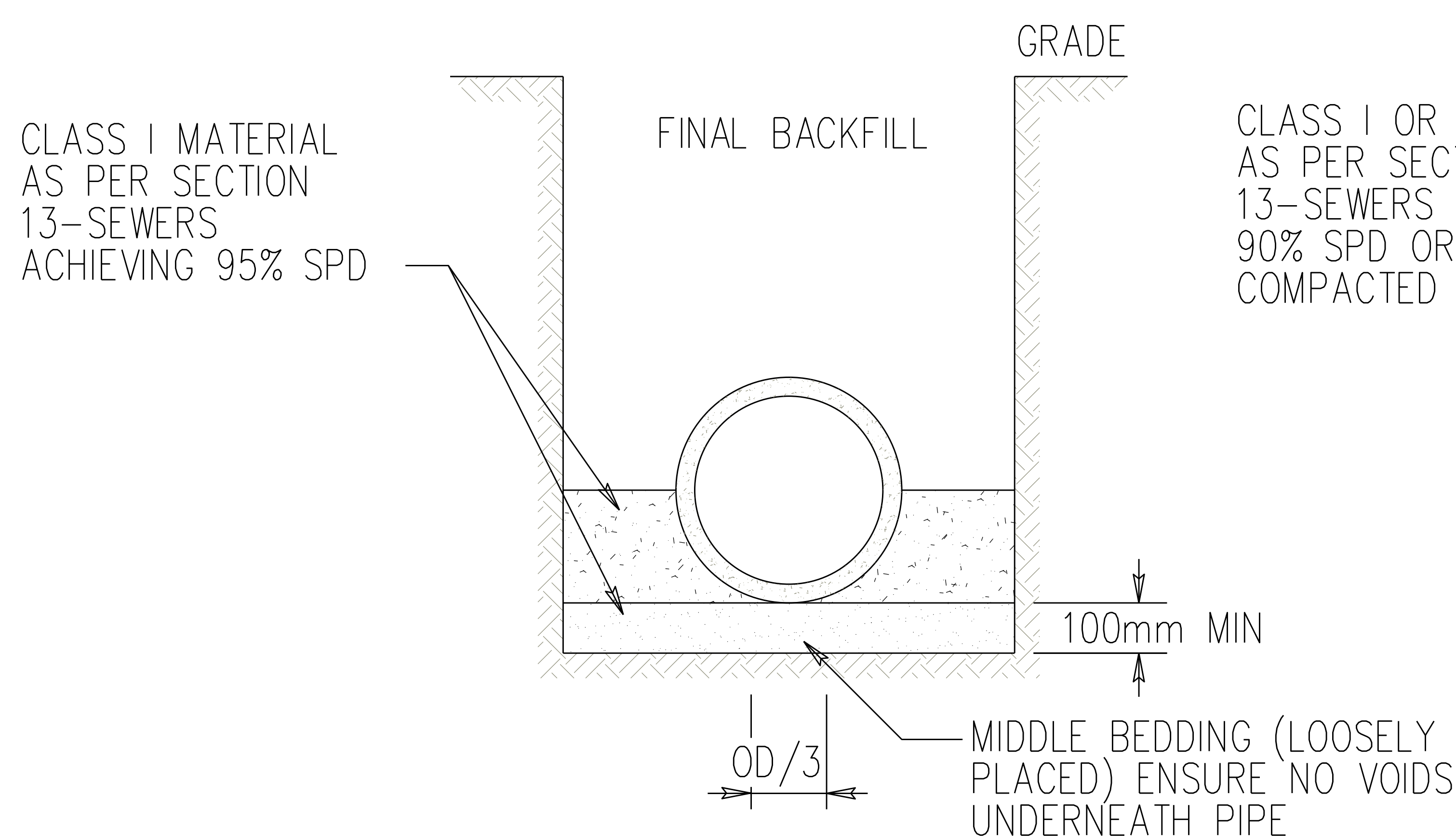
TYPE 1 INSTALLATION
