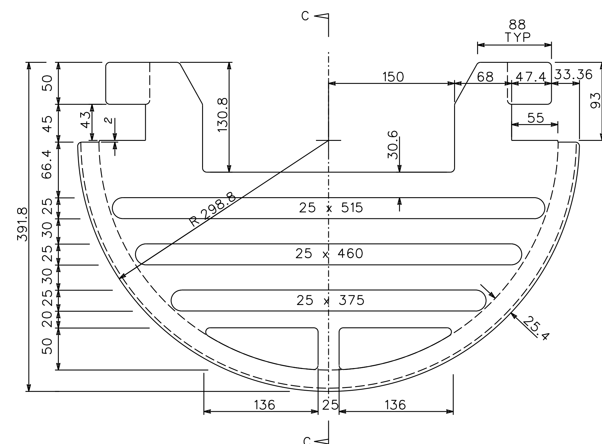
TOP VIEW - COVER (Part A) NOTE: CAST IRON MATERIAL
