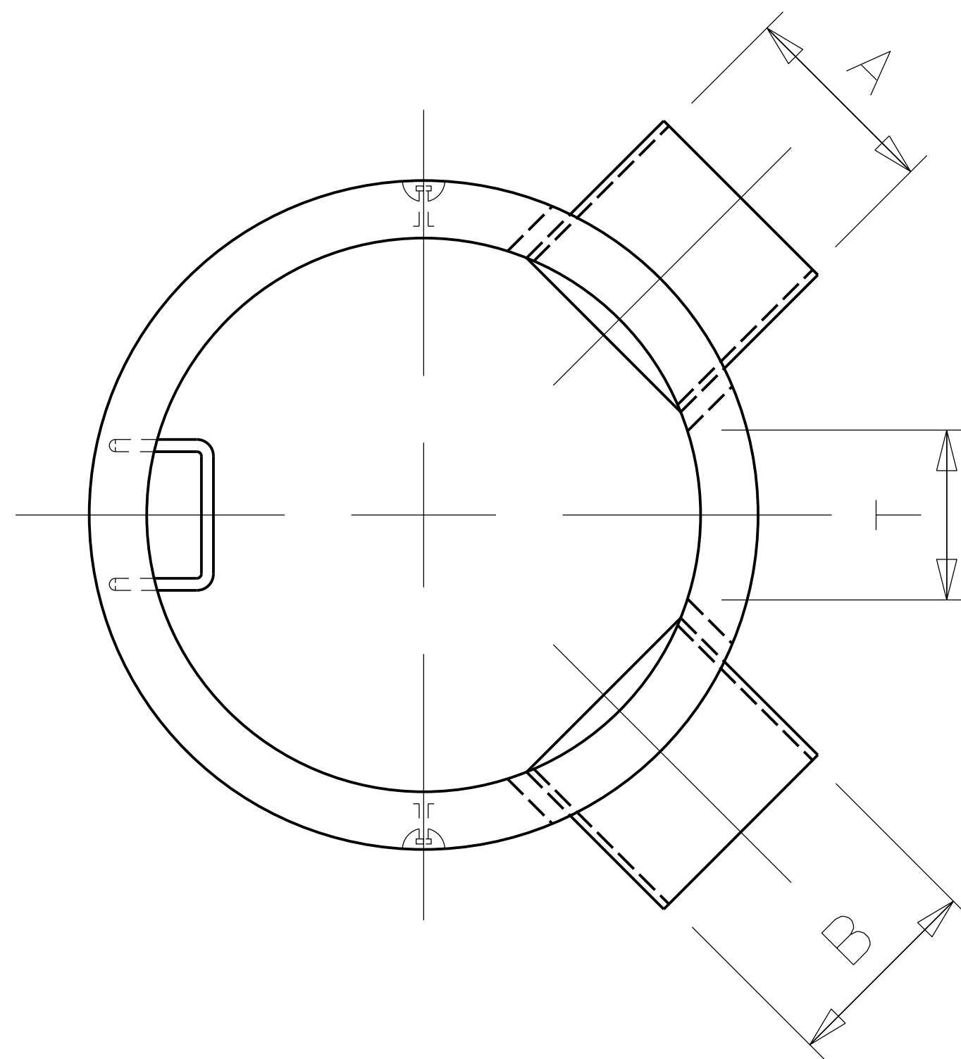
RIGHT-ANGLED 2-WAY JUNCTION
