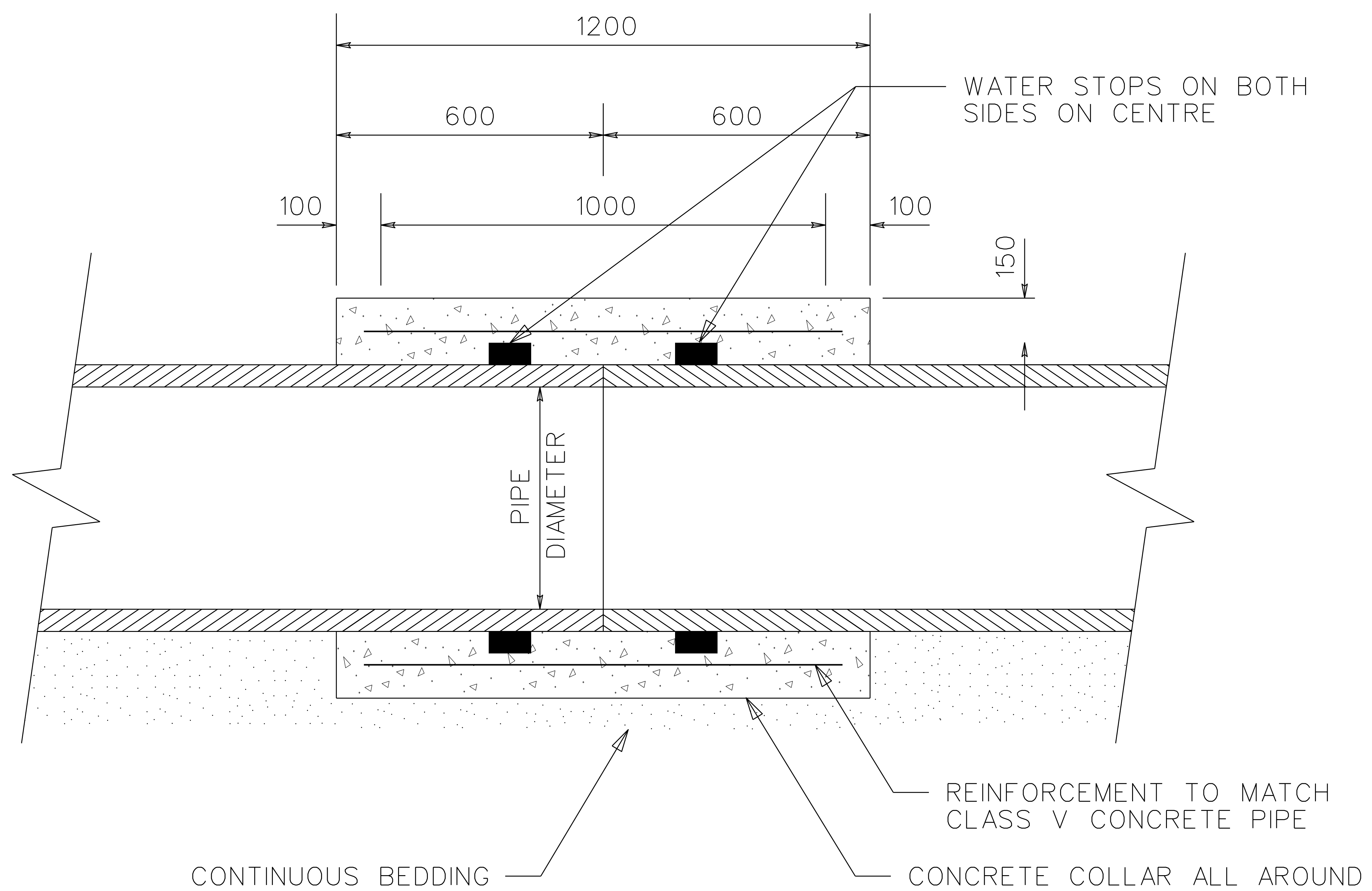
SIDE VIEW
