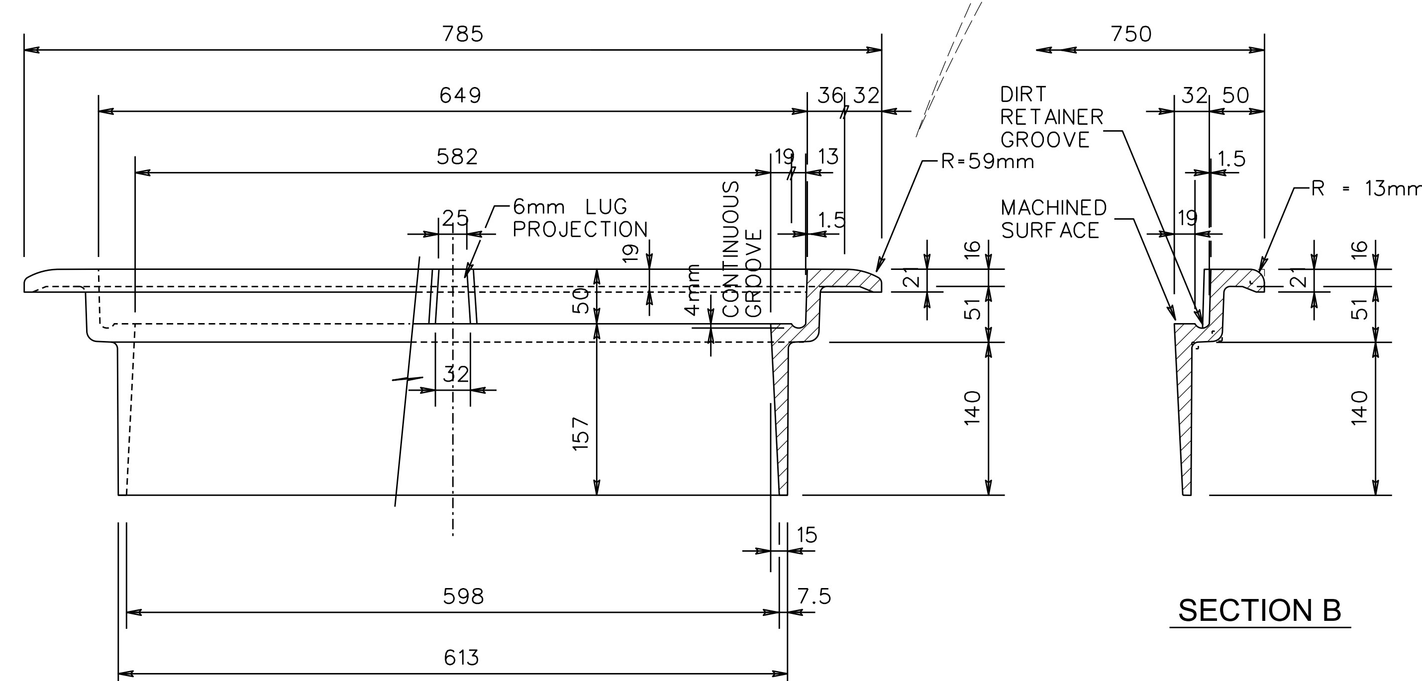
DETAIL SCALE 1:2
