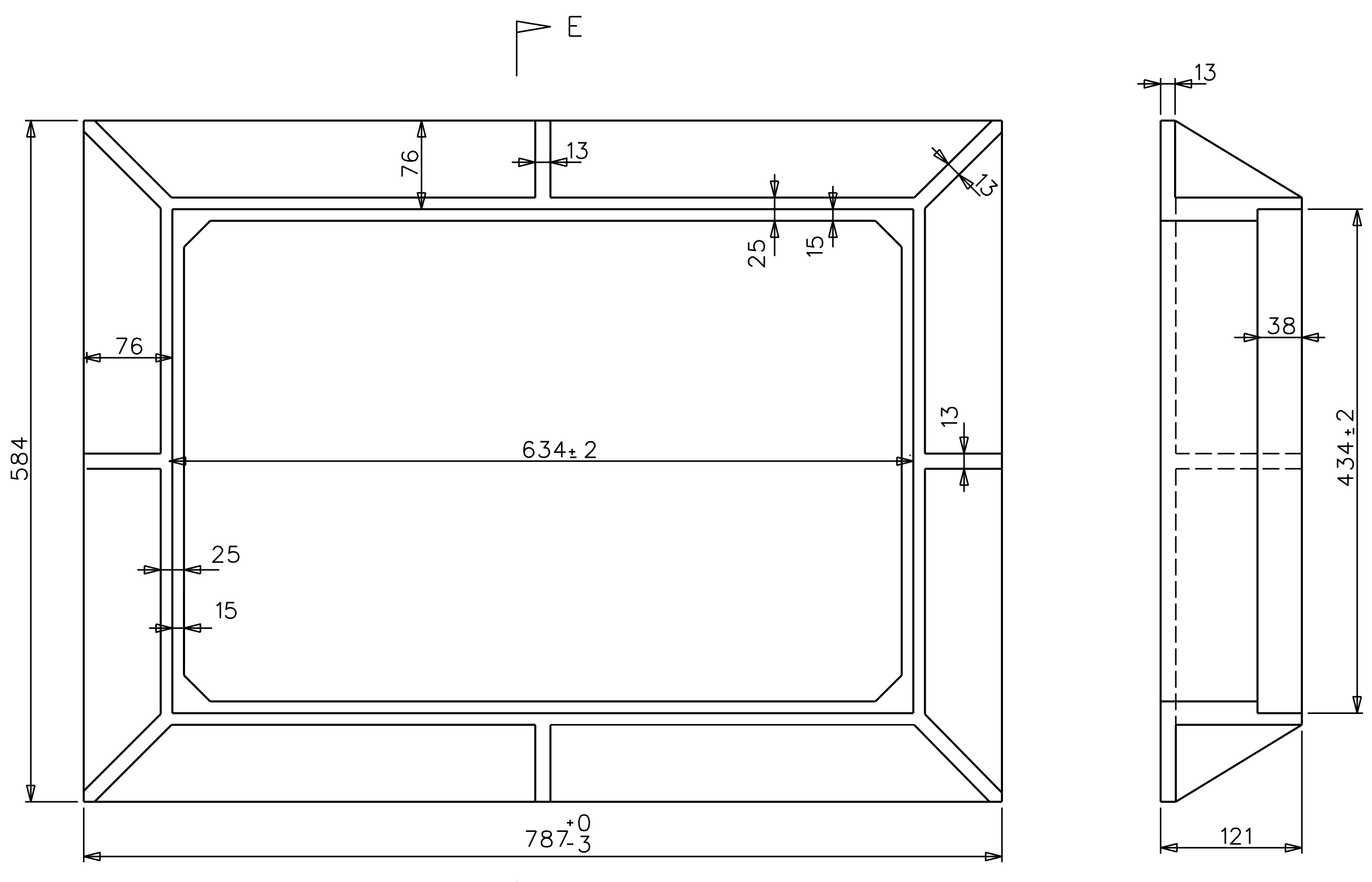
FRAME - PLAN VIEW
