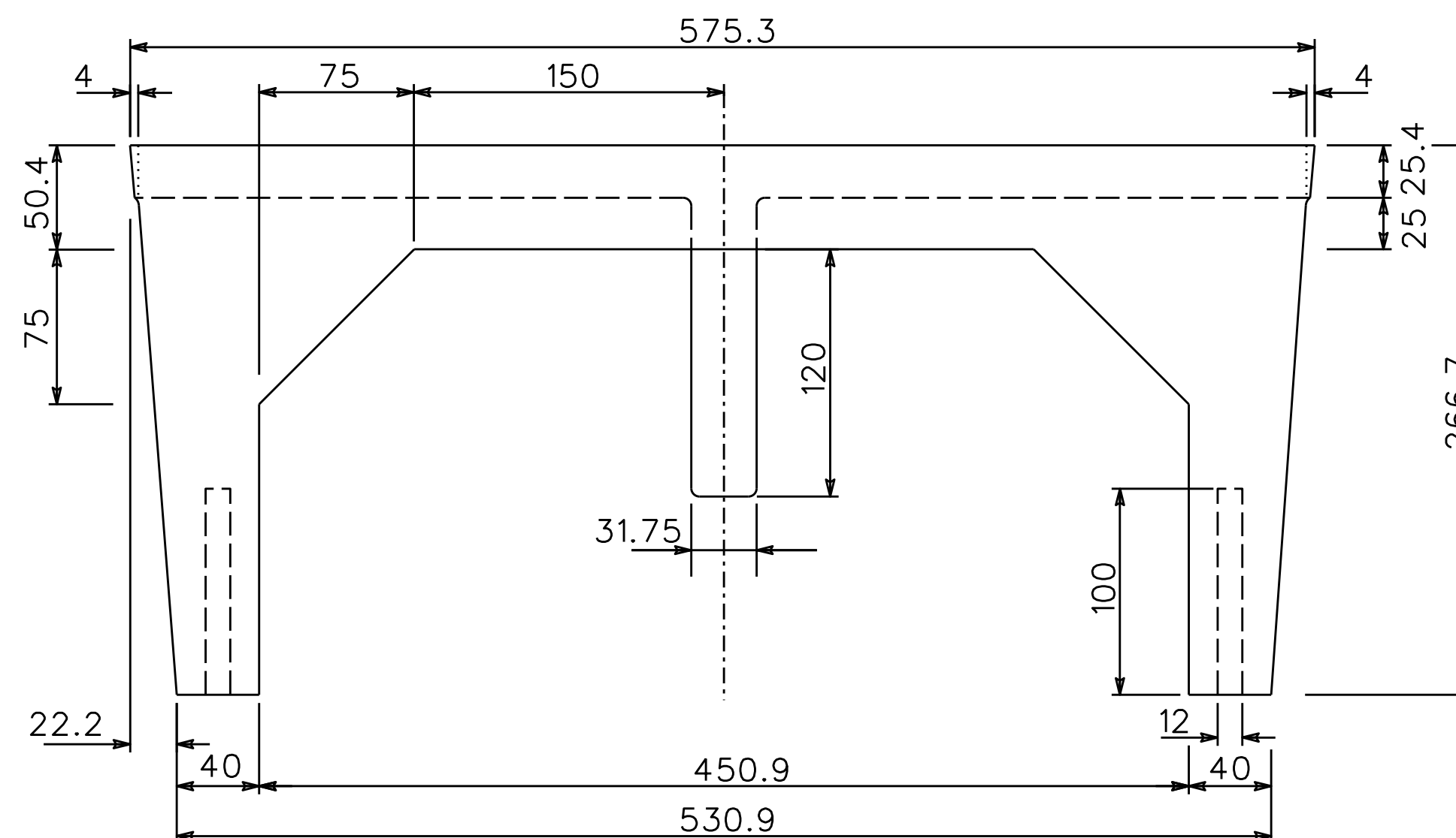
TOP VIEW - COVER (Part B)
