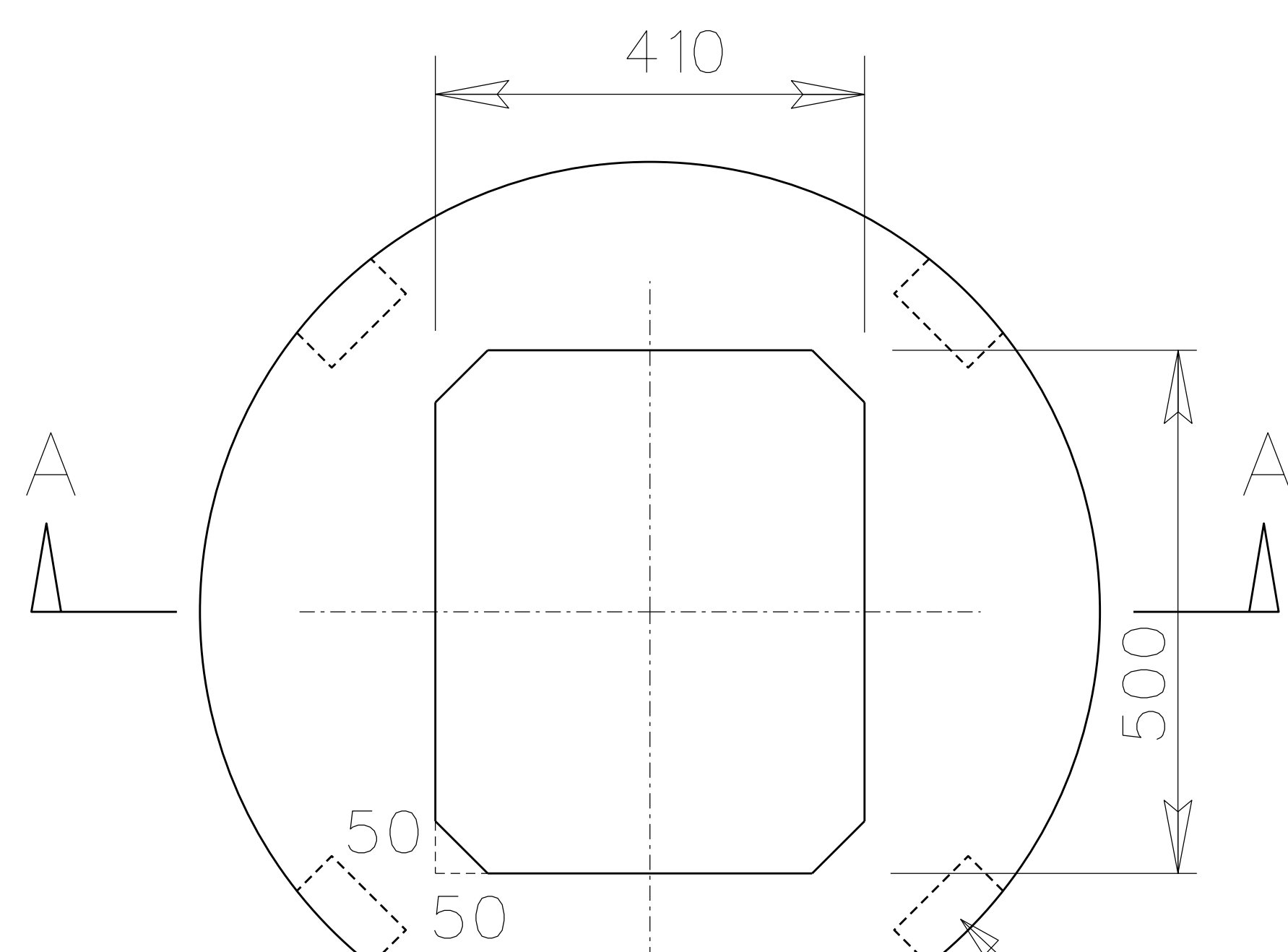
PLAN VIEW
