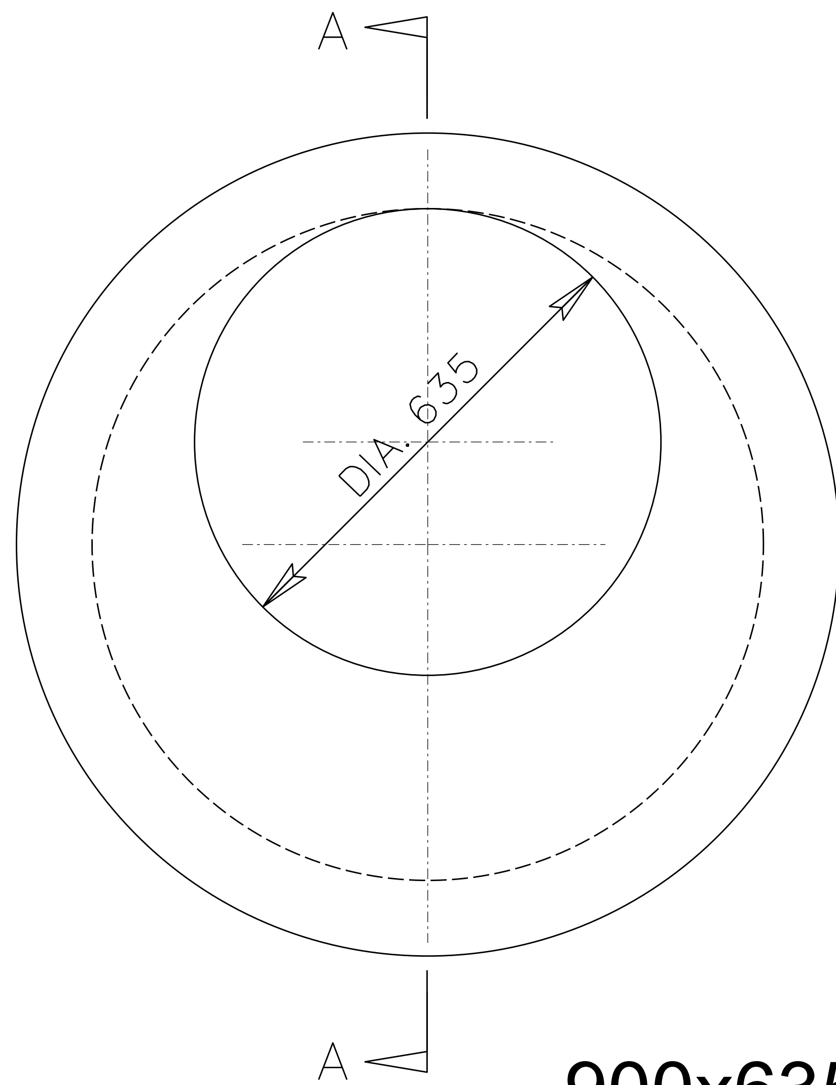
900x635 SLAB TOP
