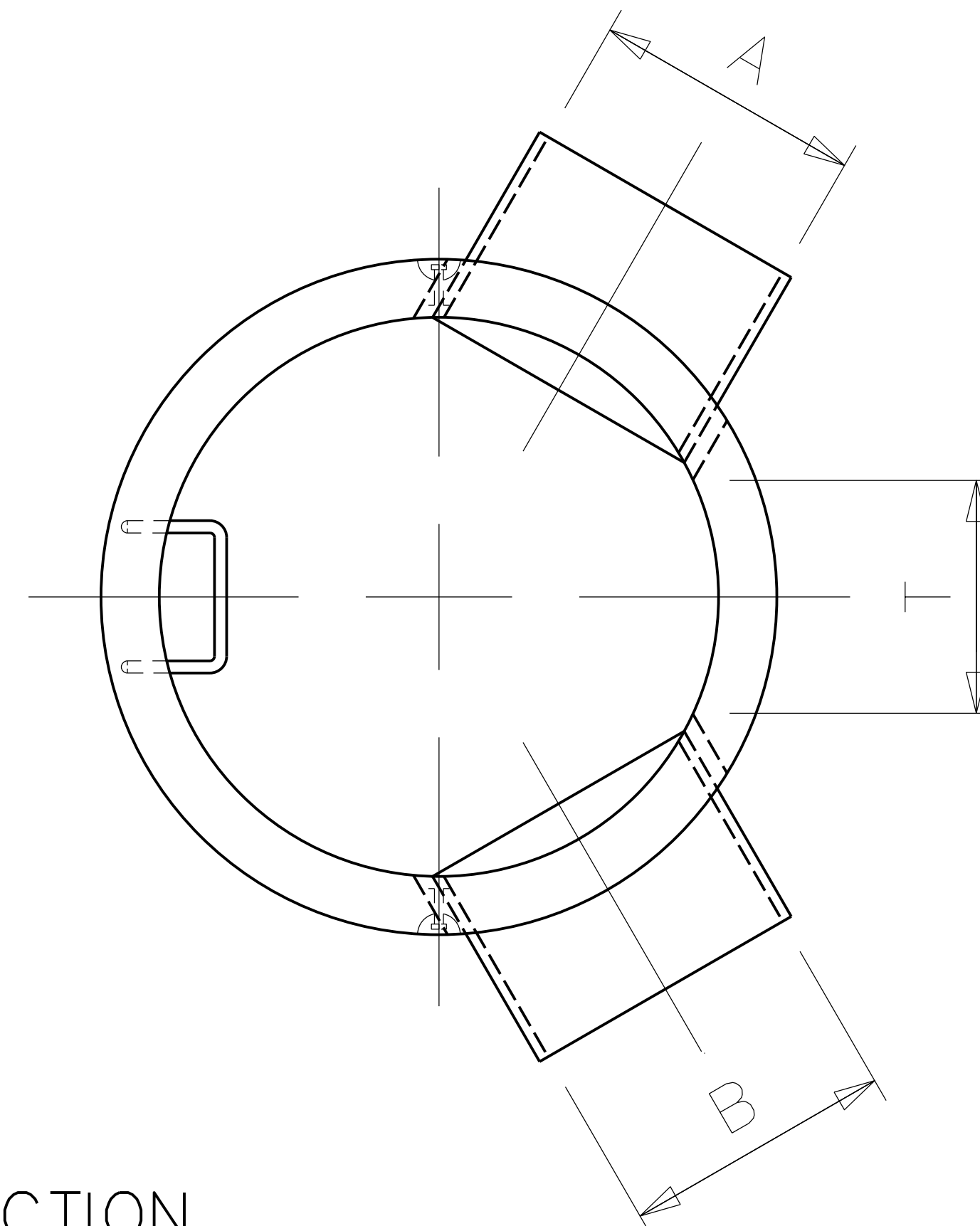
4-WAY JUNCTION
