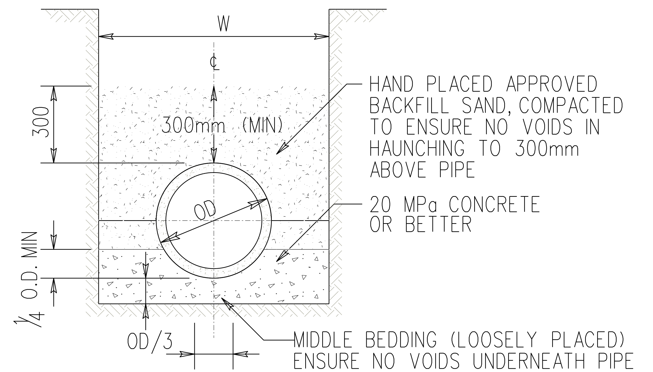
CLASS A BACKFILL (CONCRETE CRADLE)
