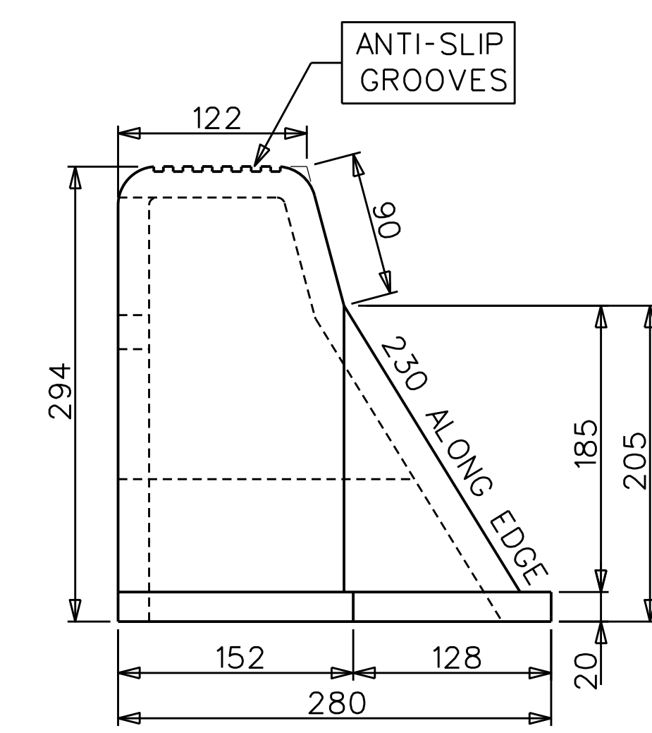
SIDE VIEW B - B
