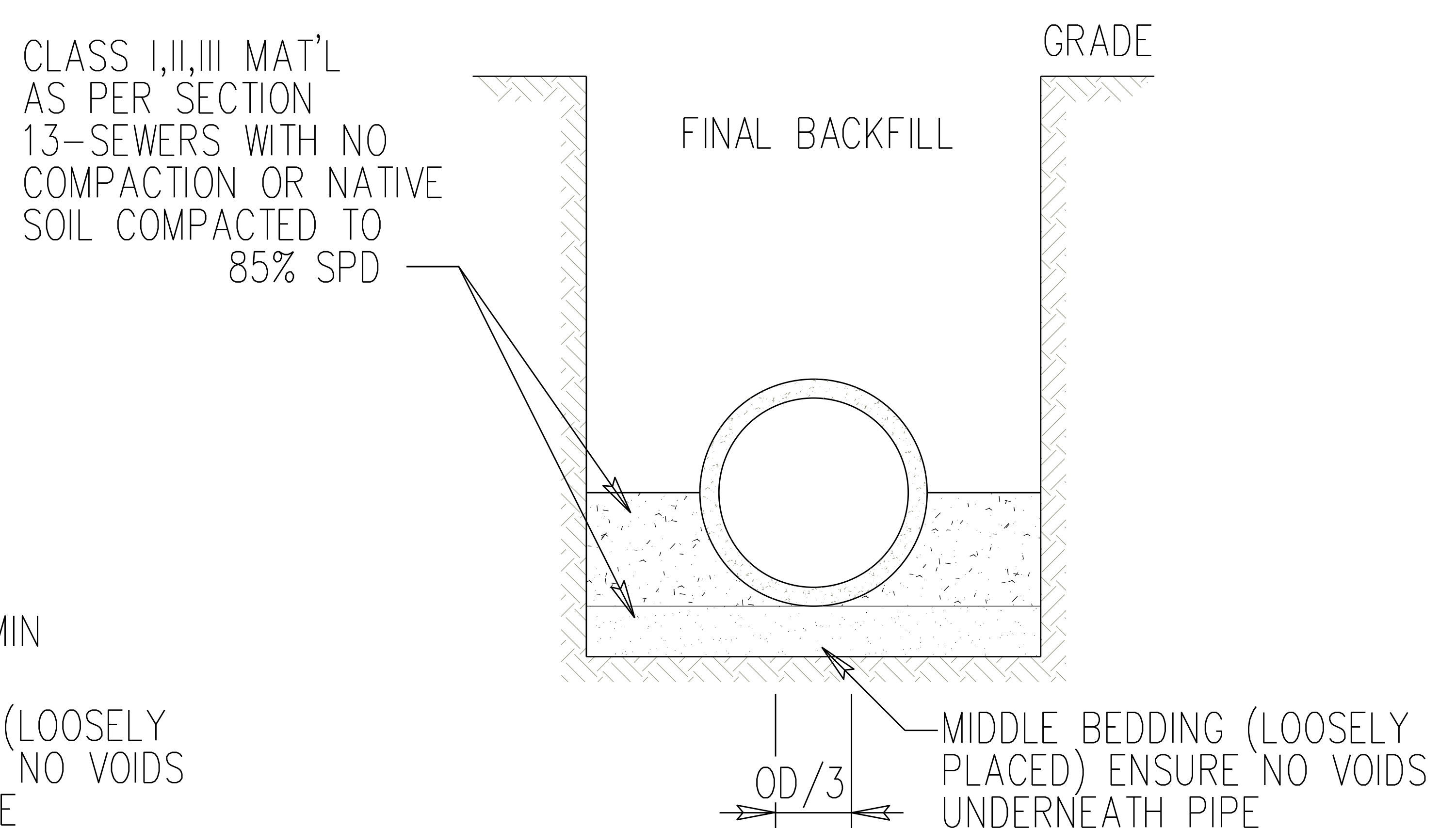
TYPE 4 INSTALLATION
