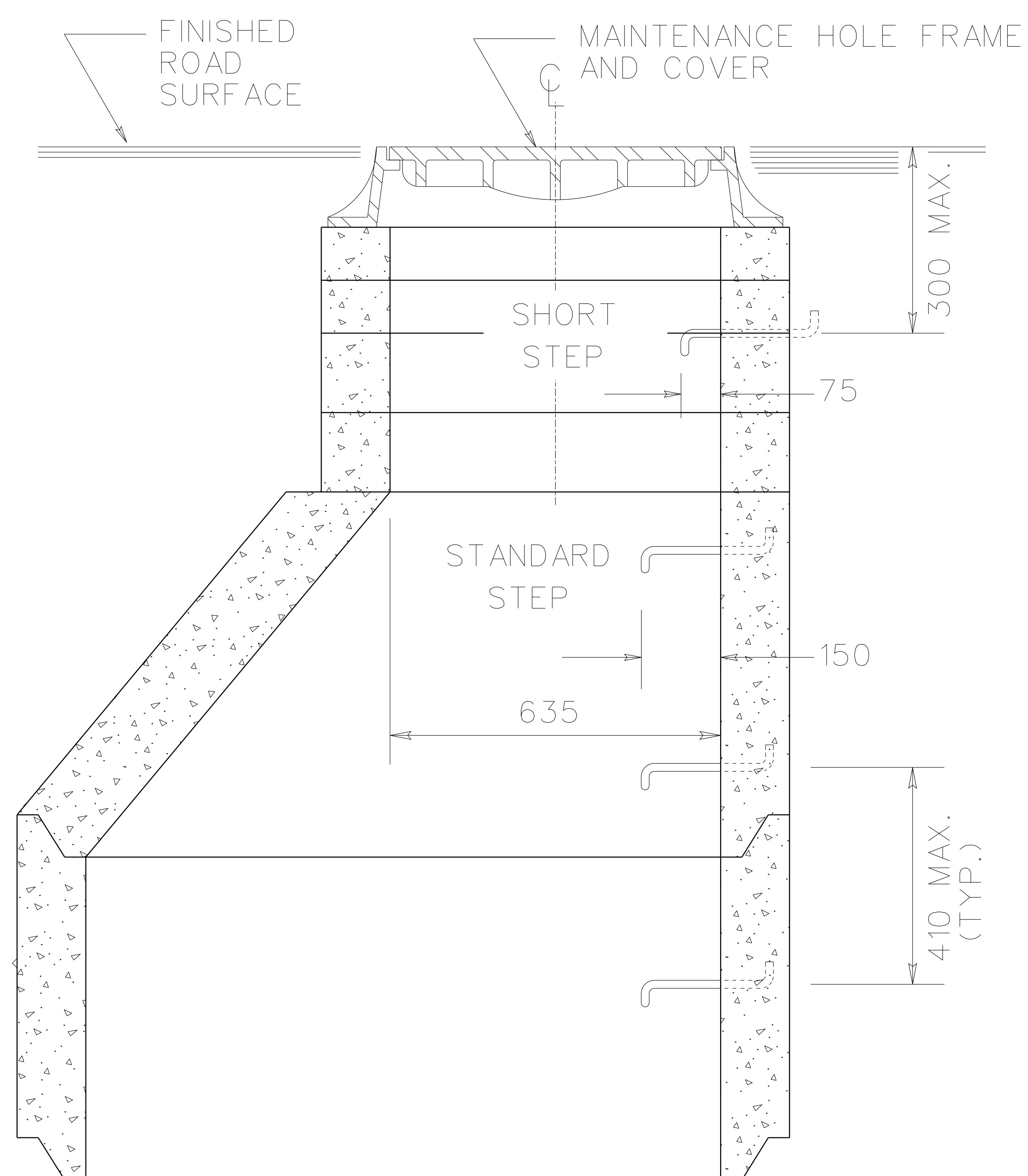
TYPICAL MAINTENANCE HOLE SECTION
