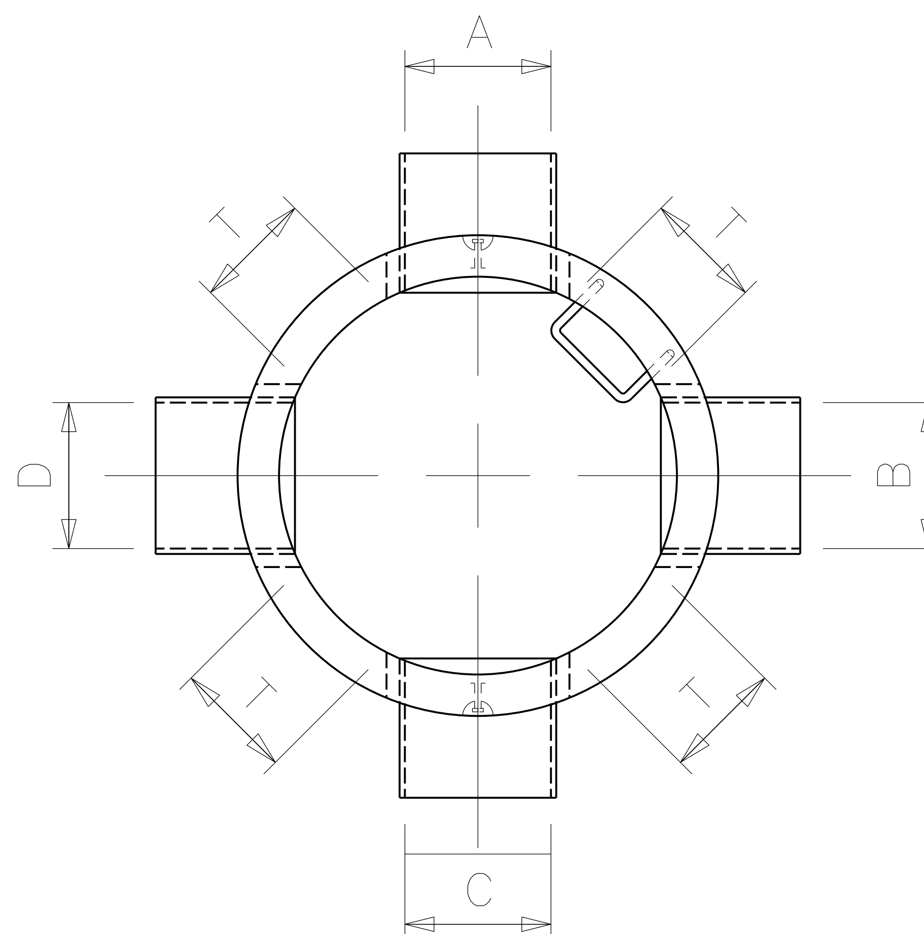
4-WAY JUNCTION
