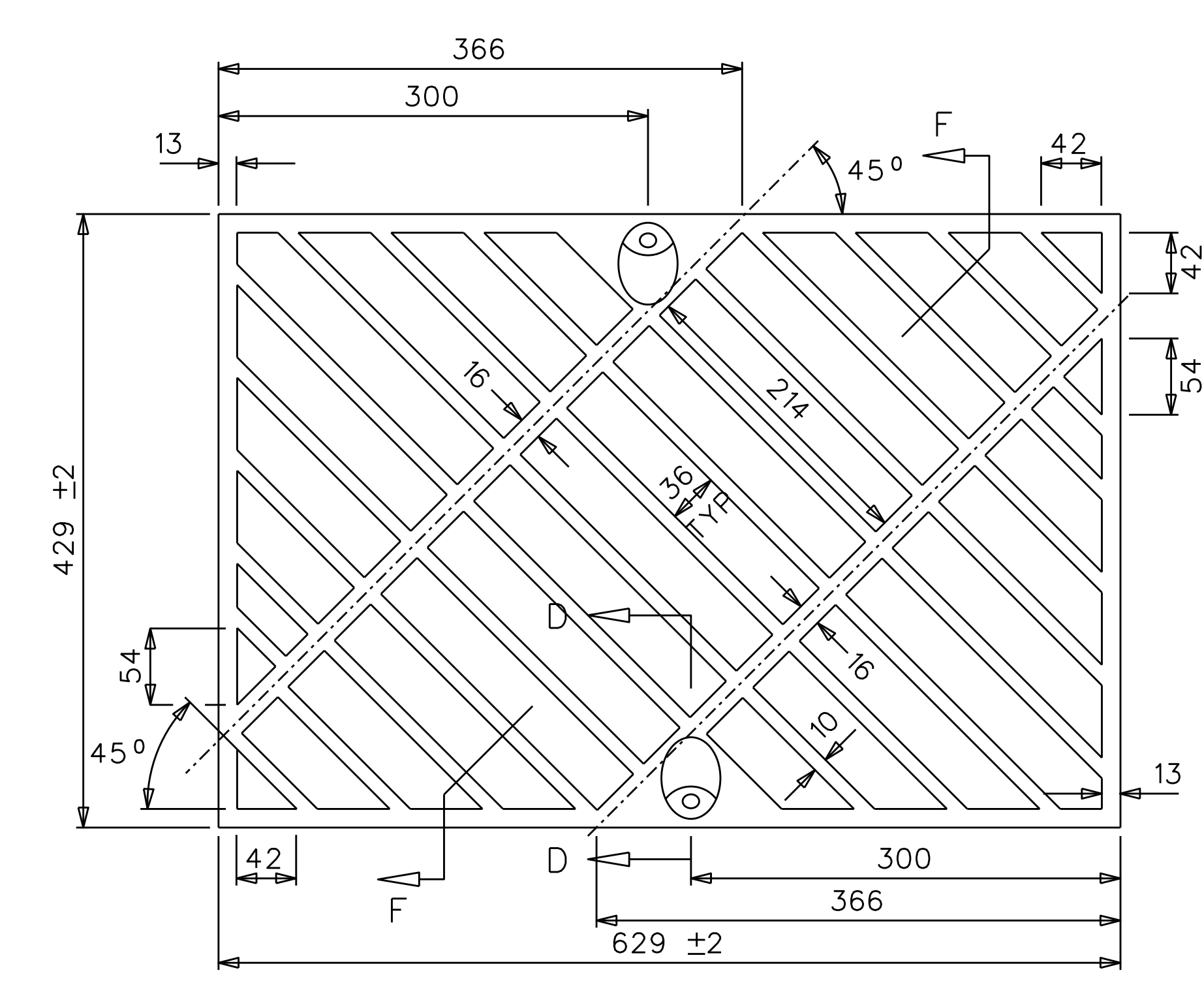
K-1 GRATE - PLAN VIEW
