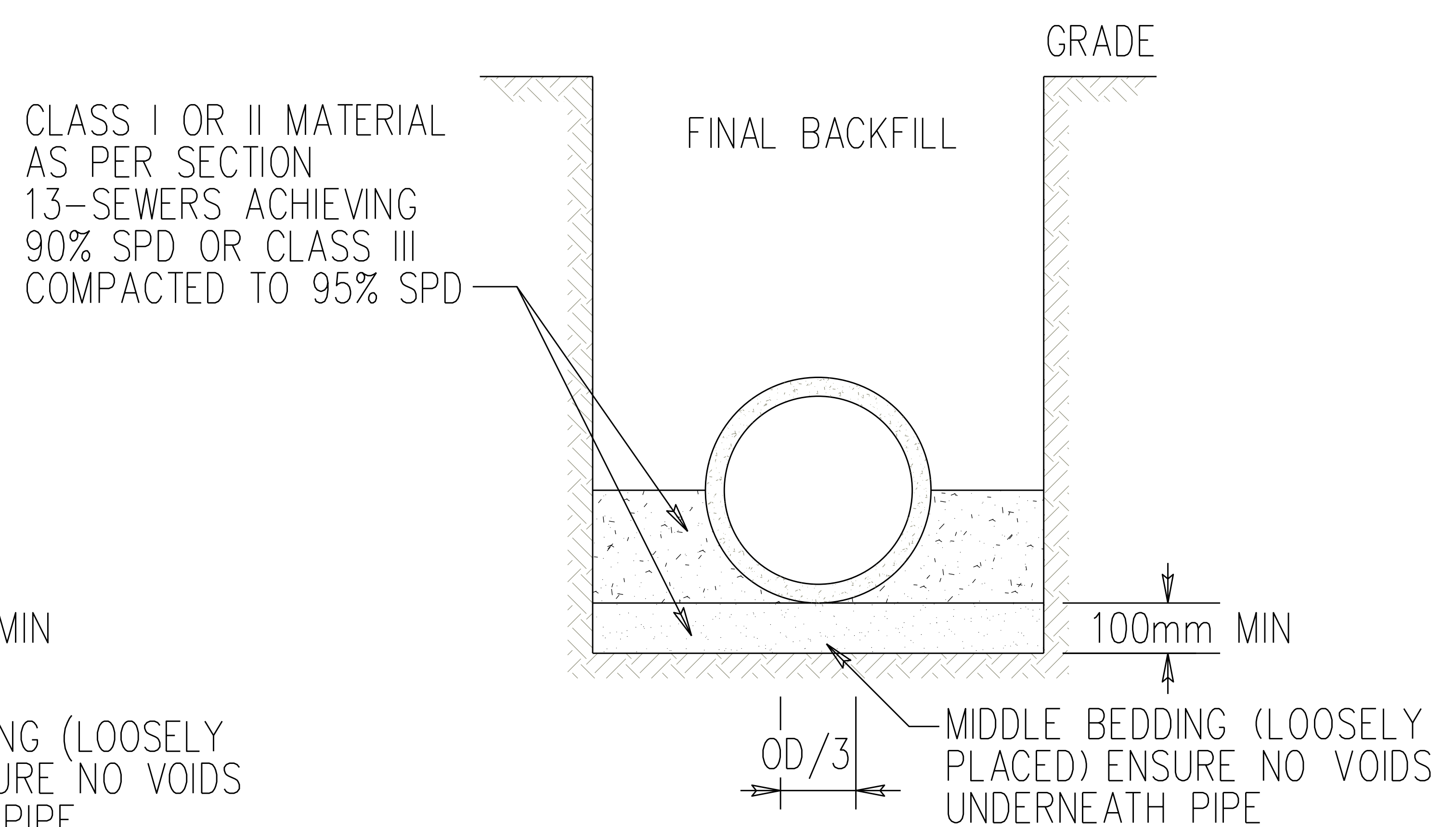
TYPE 2 INSTALLATION
